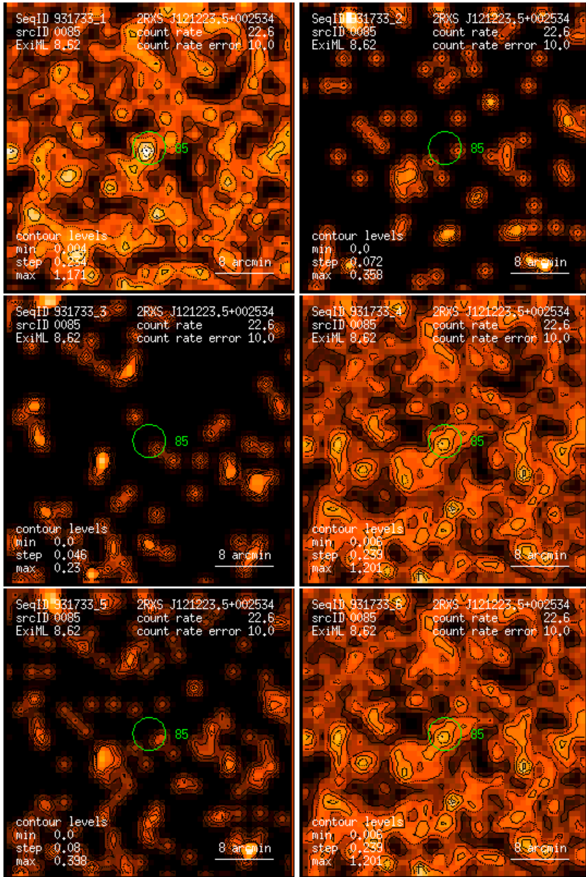
Figure 85: RASS 931733: detection 0085: band rate images, Gaussian filter: (1) PSPC channels 11 – 41, (2) 52 – 90, (3) 91 – 201, (4) 11 – 235, (5) 52 – 201, (6) 11 – 201. Broad band rates in counts/ks. Band rate contour levels in counts/ks/arcmin 2 .
