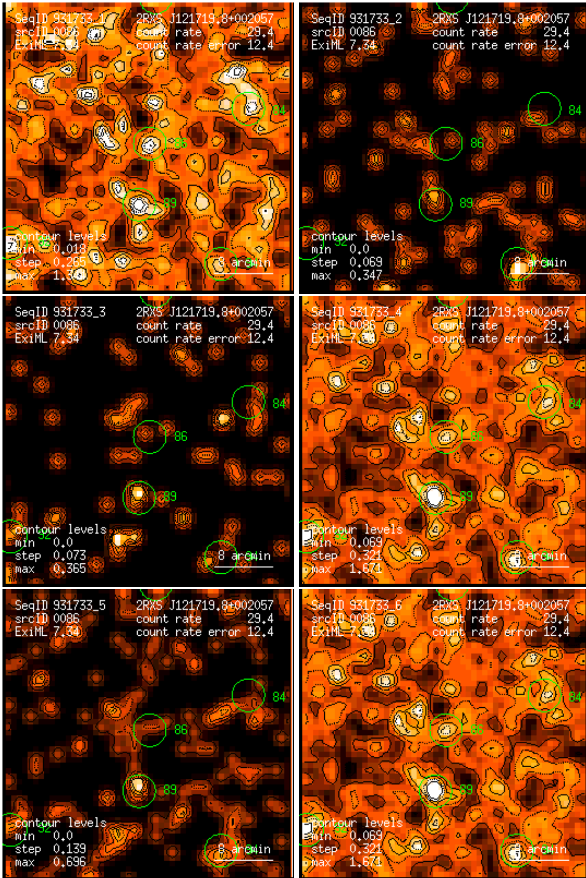
Figure 86: RASS 931733: detection 0086: band rate images, Gaussian filter: (1) PSPC channels 11 – 41, (2) 52 – 90, (3) 91 – 201, (4) 11 – 235, (5) 52 – 201, (6) 11 – 201. Broad band rates in counts/ks. Band rate contour levels in counts/ks/arcmin 2 .
