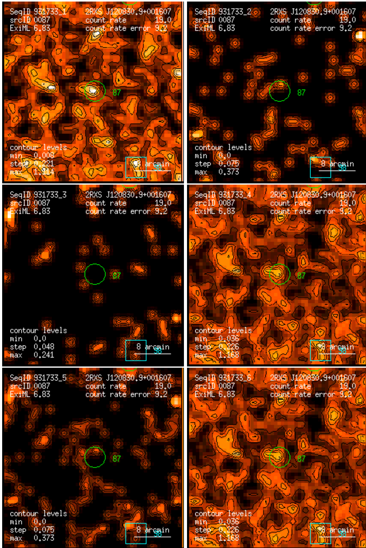
Figure 87: RASS 931733: detection 0087: band rate images, Gaussian filter: (1) PSPC channels 11 – 41, (2) 52 – 90, (3) 91 – 201, (4) 11 – 235, (5) 52 – 201, (6) 11 – 201. Broad band rates in counts/ks. Band rate contour levels in counts/ks/arcmin 2 .
