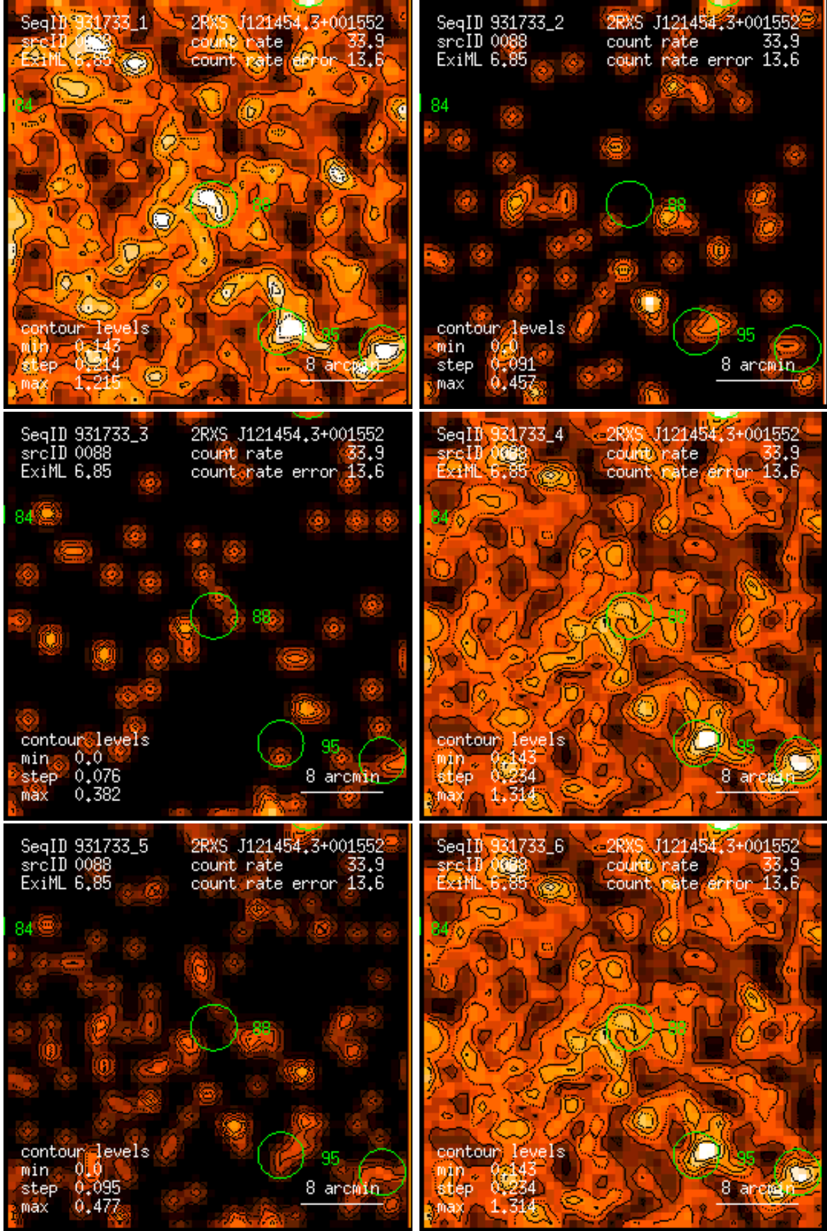
Figure 88: RASS 931733: detection 0088: band rate images, Gaussian filter: (1) PSPC channels 11 – 41, (2) 52 – 90, (3) 91 – 201, (4) 11 – 235, (5) 52 – 201, (6) 11 – 201. Broad band rates in counts/ks. Band rate contour levels in counts/ks/arcmin 2 .
