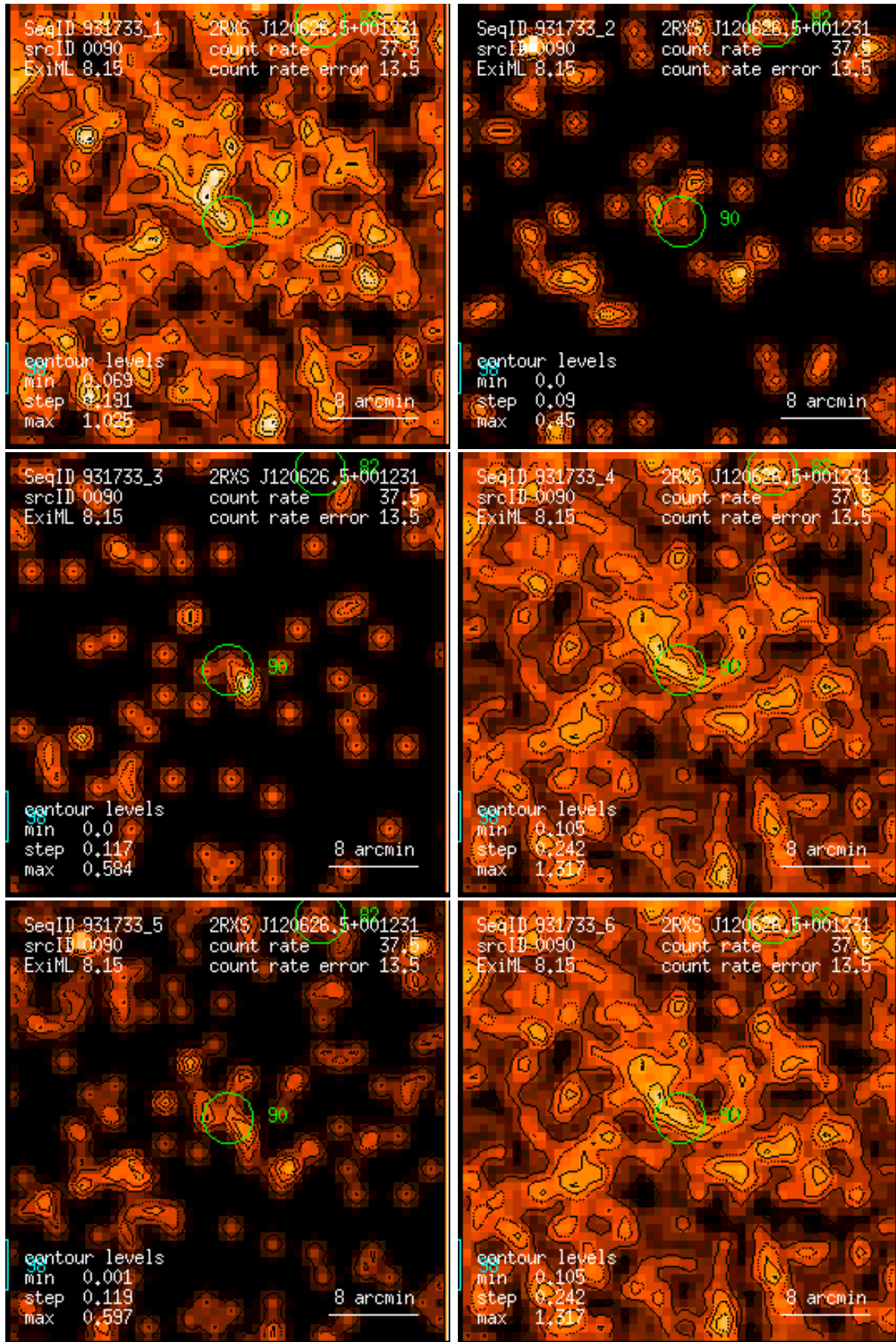
Figure 90: RASS 931733: detection 0090: band rate images, Gaussian filter: (1) PSPC channels 11 – 41, (2) 52 – 90, (3) 91 – 201, (4) 11 – 235, (5) 52 – 201, (6) 11 – 201. Broad band rates in counts/ks. Band rate contour levels in counts/ks/arcmin 2 .
