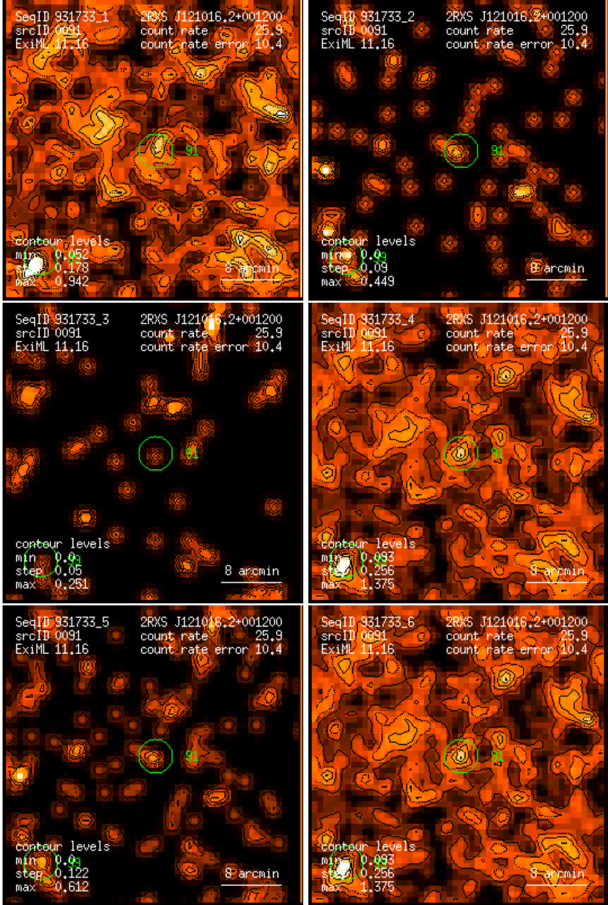
Figure 91: RASS 931733: detection 0091: band rate images, Gaussian filter: (1) PSPC channels 11 – 41, (2) 52 – 90, (3) 91 – 201, (4) 11 – 235, (5) 52 – 201, (6) 11 – 201. Broad band rates in counts/ks. Band rate contour levels in counts/ks/arcmin 2 .
