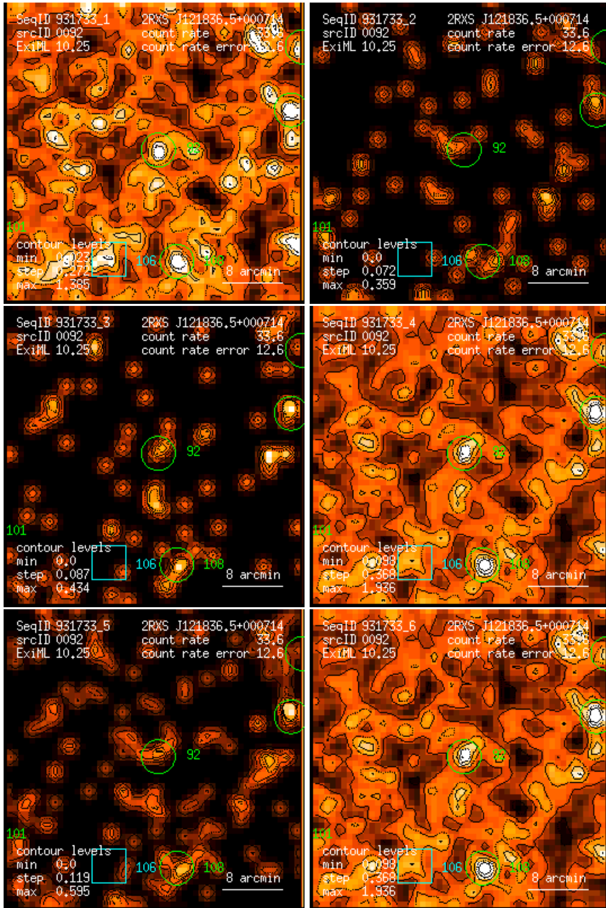
Figure 92: RASS 931733: detection 0092: band rate images, Gaussian filter: (1) PSPC channels 11 – 41, (2) 52 – 90, (3) 91 – 201, (4) 11 – 235, (5) 52 – 201, (6) 11 – 201. Broad band rates in counts/ks. Band rate contour levels in counts/ks/arcmin 2 .
