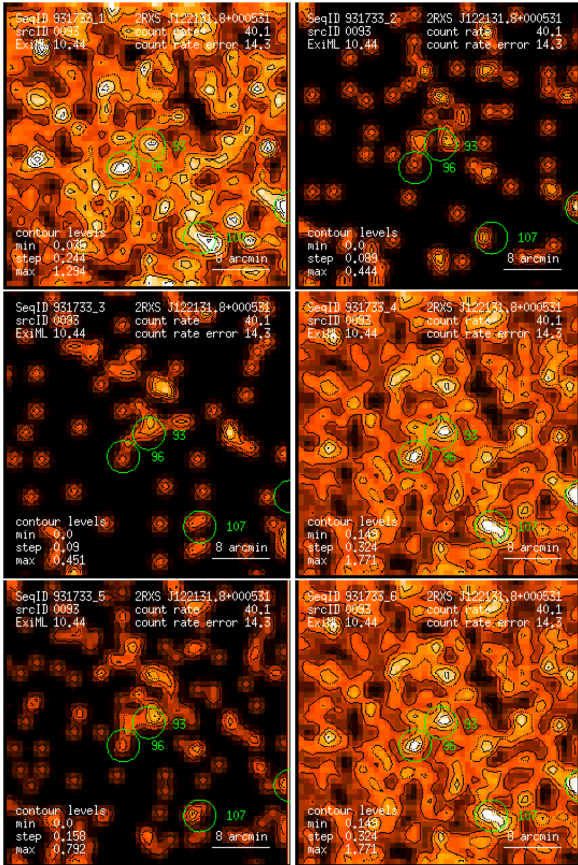
Figure 93: RASS 931733: detection 0093: band rate images, Gaussian filter: (1) PSPC channels 11 – 41, (2) 52 – 90, (3) 91 – 201, (4) 11 – 235, (5) 52 – 201, (6) 11 – 201. Broad band rates in counts/ks. Band rate contour levels in counts/ks/arcmin 2 .
