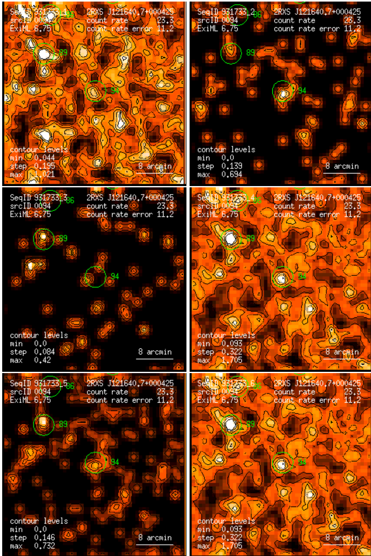
Figure 94: RASS 931733: detection 0094: band rate images, Gaussian filter: (1) PSPC channels 11 – 41, (2) 52 – 90, (3) 91 – 201, (4) 11 – 235, (5) 52 – 201, (6) 11 – 201. Broad band rates in counts/ks. Band rate contour levels in counts/ks/arcmin 2 .
