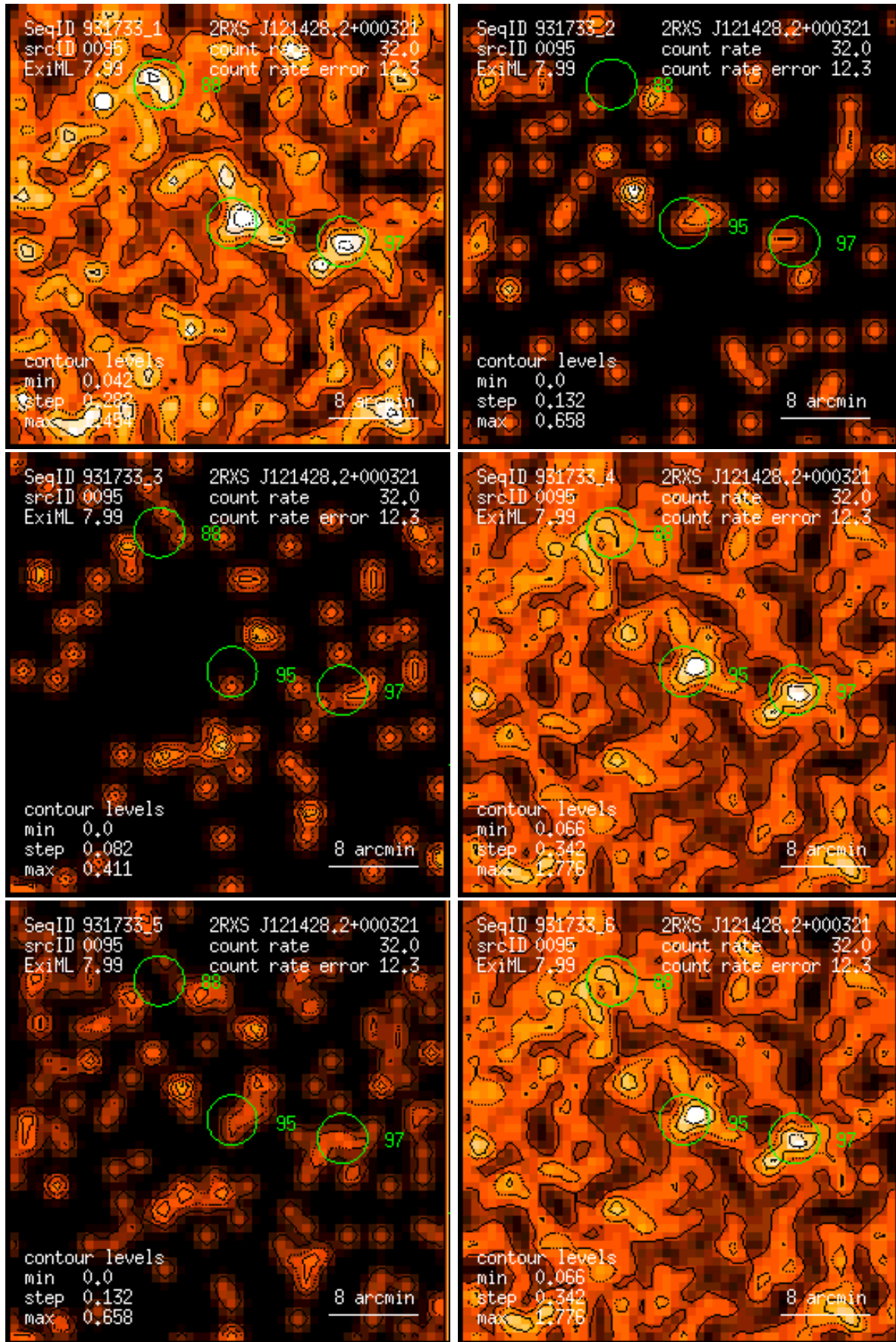
Figure 95: RASS 931733: detection 0095: band rate images, Gaussian filter: (1) PSPC channels 11 – 41, (2) 52 – 90, (3) 91 – 201, (4) 11 – 235, (5) 52 – 201, (6) 11 – 201. Broad band rates in counts/ks. Band rate contour levels in counts/ks/arcmin 2 .
