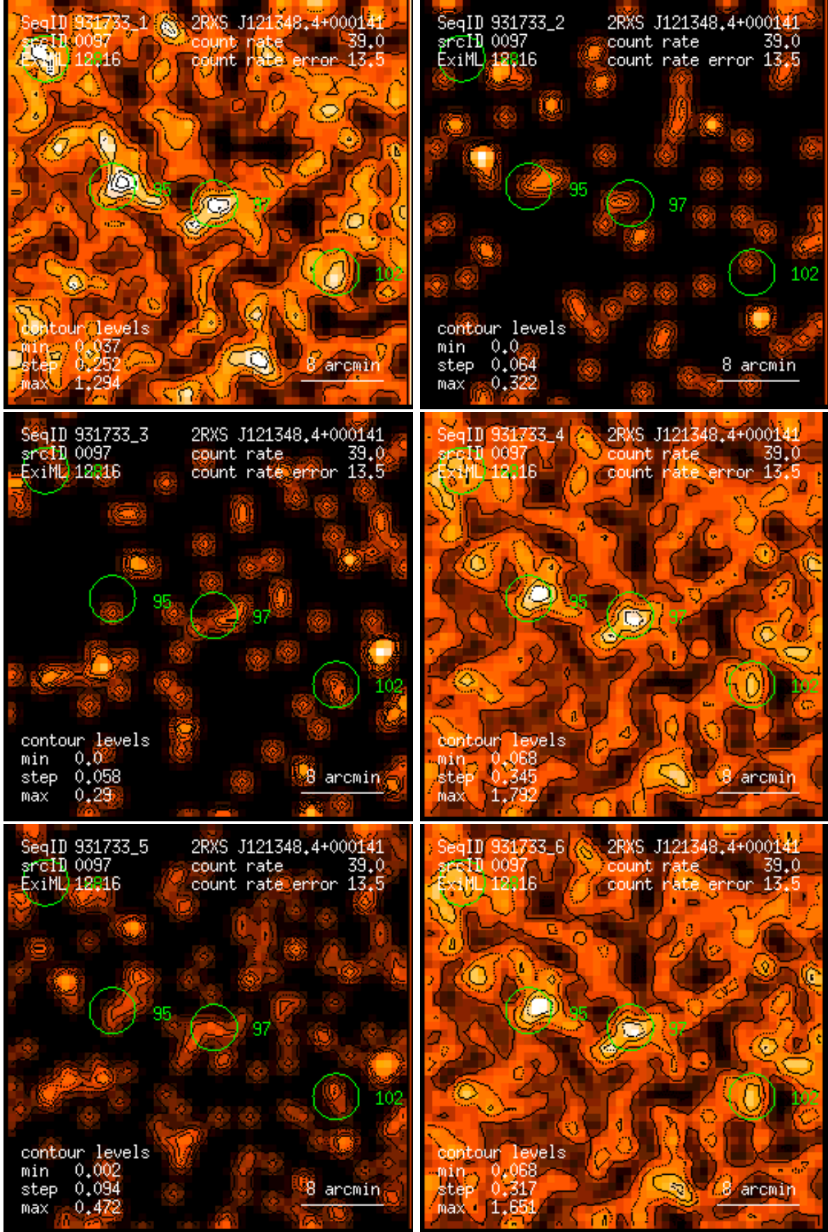
Figure 97: RASS 931733: detection 0097: band rate images, Gaussian filter: (1) PSPC channels 11 – 41, (2) 52 – 90, (3) 91 – 201, (4) 11 – 235, (5) 52 – 201, (6) 11 – 201. Broad band rates in counts/ks. Band rate contour levels in counts/ks/arcmin 2 .
