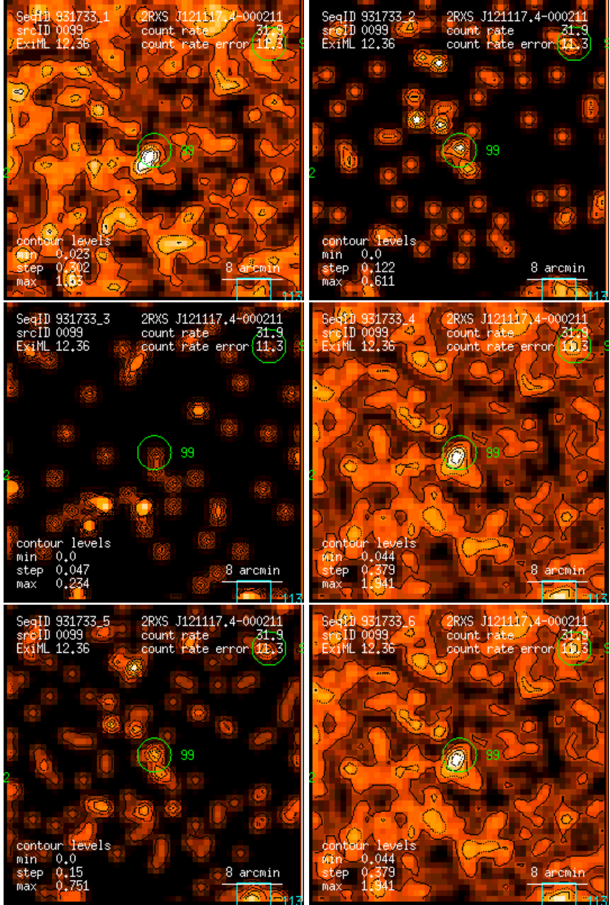
Figure 99: RASS 931733: detection 0099: band rate images, Gaussian filter: (1) PSPC channels 11 – 41, (2) 52 – 90, (3) 91 – 201, (4) 11 – 235, (5) 52 – 201, (6) 11 – 201. Broad band rates in counts/ks. Band rate contour levels in counts/ks/arcmin 2 .
