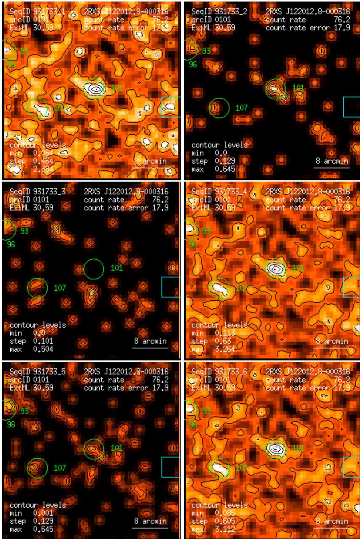
Figure 101: RASS 931733: detection 0101: band rate images, Gaussian filter: (1) PSPC channels 11 – 41, (2) 52 – 90, (3) 91 – 201, (4) 11 – 235, (5) 52 – 201, (6) 11 – 201. Broad band rates in counts/ks. Band rate contour levels in counts/ks/arcmin 2 .
