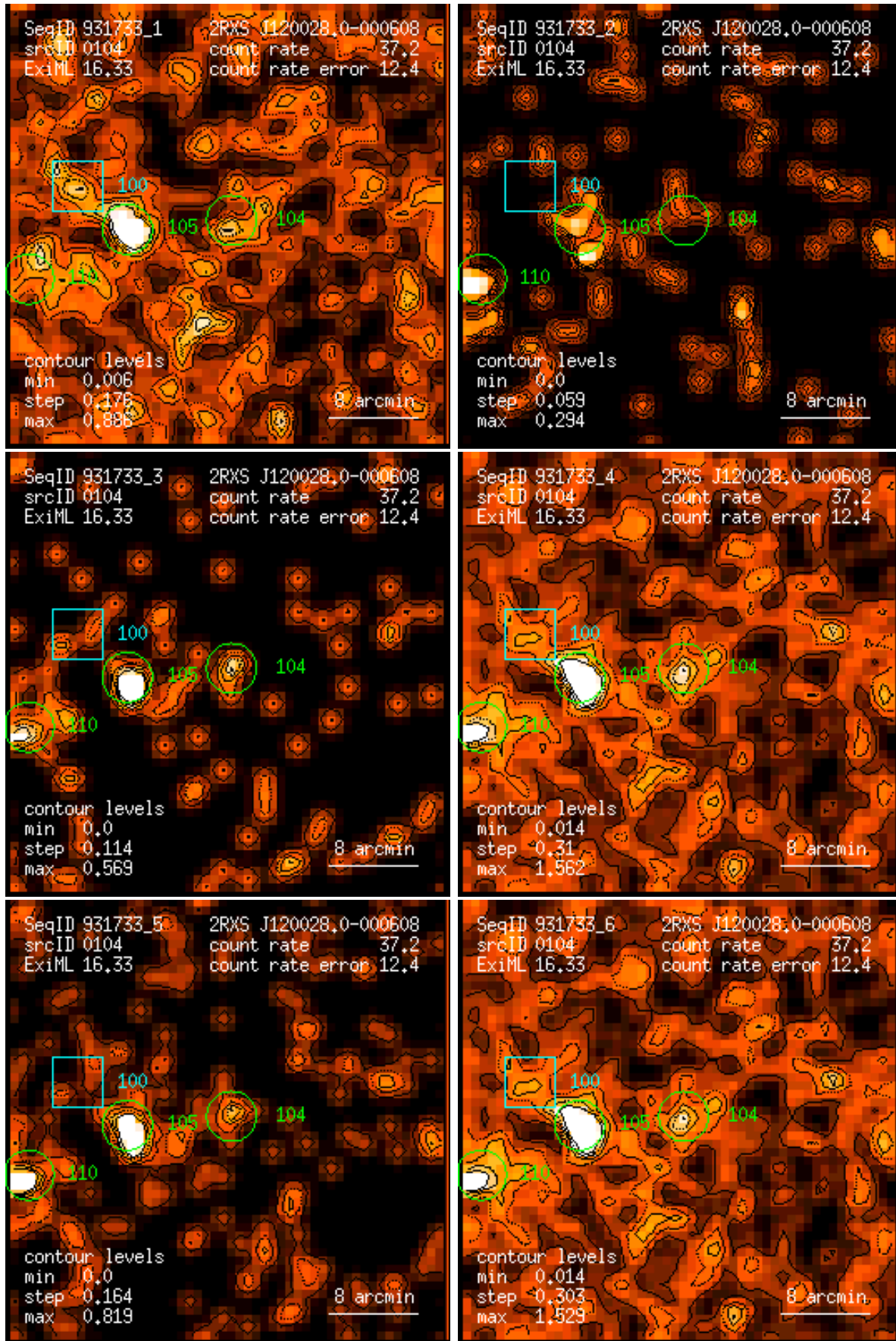
Figure 104: RASS 931733: detection 0104: band rate images, Gaussian filter: (1) PSPC channels 11 – 41, (2) 52 – 90, (3) 91 – 201, (4) 11 – 235, (5) 52 – 201, (6) 11 – 201. Broad band rates in counts/ks. Band rate contour levels in counts/ks/arcmin 2 .
