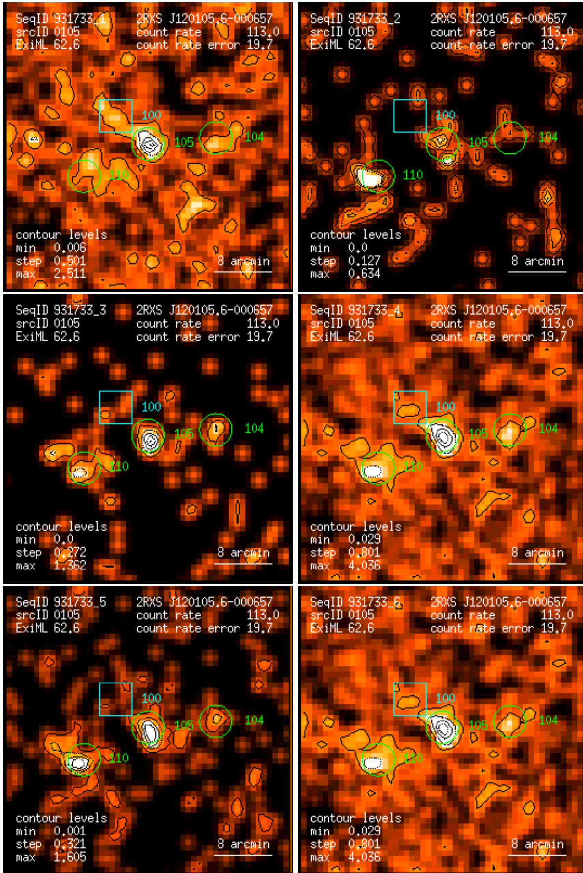
Figure 105: RASS 931733: detection 0105: band rate images, Gaussian filter: (1) PSPC channels 11 – 41, (2) 52 – 90, (3) 91 – 201, (4) 11 – 235, (5) 52 – 201, (6) 11 – 201. Broad band rates in counts/ks. Band rate contour levels in counts/ks/arcmin 2 .
