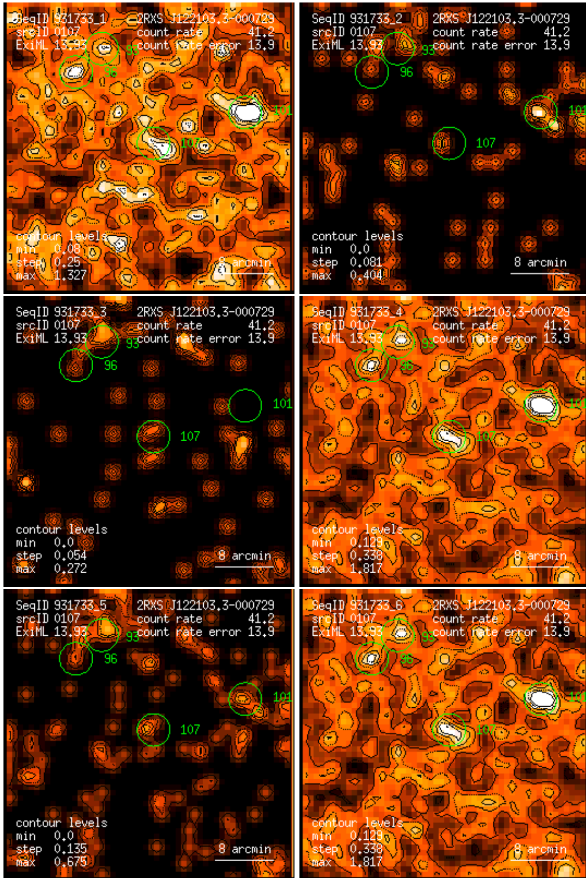
Figure 107: RASS 931733: detection 0107: band rate images, Gaussian filter: (1) PSPC channels 11 – 41, (2) 52 – 90, (3) 91 – 201, (4) 11 – 235, (5) 52 – 201, (6) 11 – 201. Broad band rates in counts/ks. Band rate contour levels in counts/ks/arcmin 2 .
