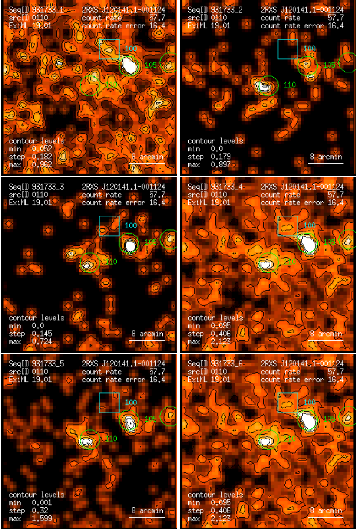
Figure 110: RASS 931733: detection 0110: band rate images, Gaussian filter: (1) PSPC channels 11 – 41, (2) 52 – 90, (3) 91 – 201, (4) 11 – 235, (5) 52 – 201, (6) 11 – 201. Broad band rates in counts/ks. Band rate contour levels in counts/ks/arcmin 2 .
