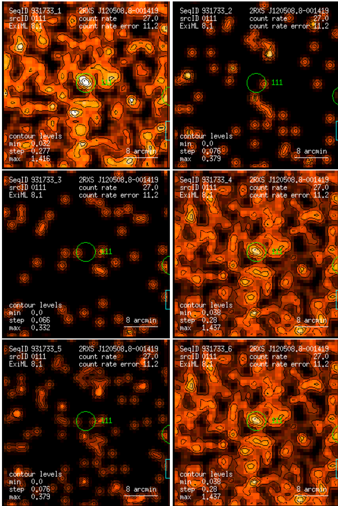
Figure 111: RASS 931733: detection 0111: band rate images, Gaussian filter: (1) PSPC channels 11 – 41, (2) 52 – 90, (3) 91 – 201, (4) 11 – 235, (5) 52 – 201, (6) 11 – 201. Broad band rates in counts/ks. Band rate contour levels in counts/ks/arcmin 2 .
