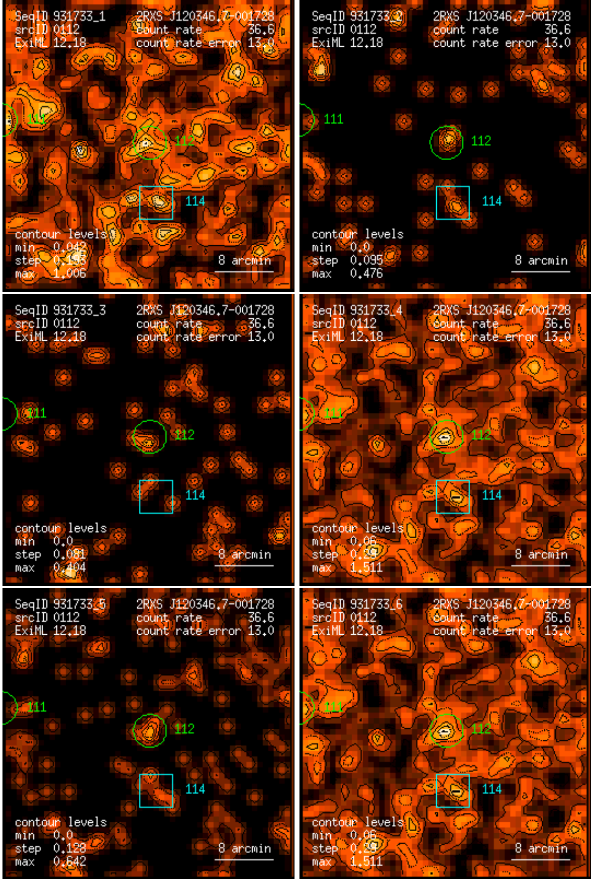
Figure 112: RASS 931733: detection 0112: band rate images, Gaussian filter: (1) PSPC channels 11 – 41, (2) 52 – 90, (3) 91 – 201, (4) 11 – 235, (5) 52 – 201, (6) 11 – 201. Broad band rates in counts/ks. Band rate contour levels in counts/ks/arcmin 2 .
