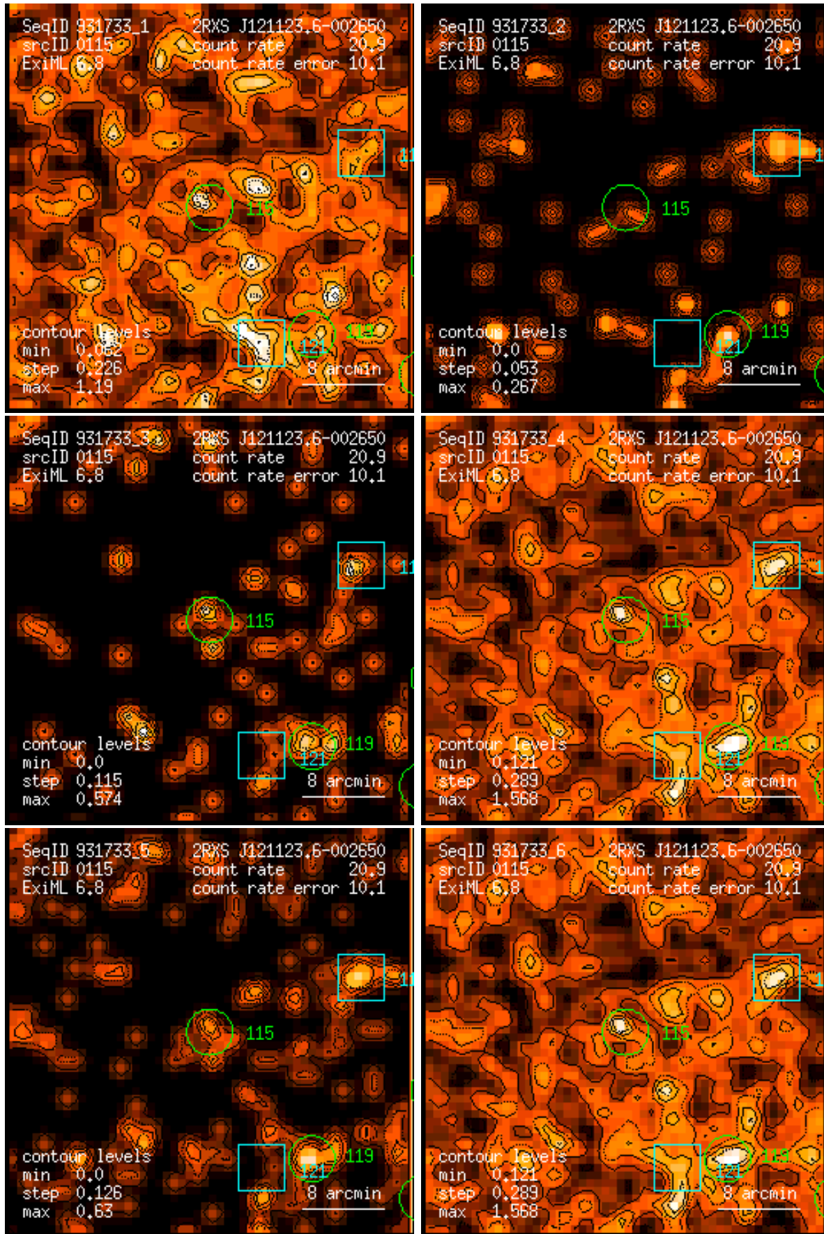
Figure 115: RASS 931733: detection 0115: band rate images, Gaussian filter: (1) PSPC channels 11 – 41, (2) 52 – 90, (3) 91 – 201, (4) 11 – 235, (5) 52 – 201, (6) 11 – 201. Broad band rates in counts/ks. Band rate contour levels in counts/ks/arcmin 2 .
