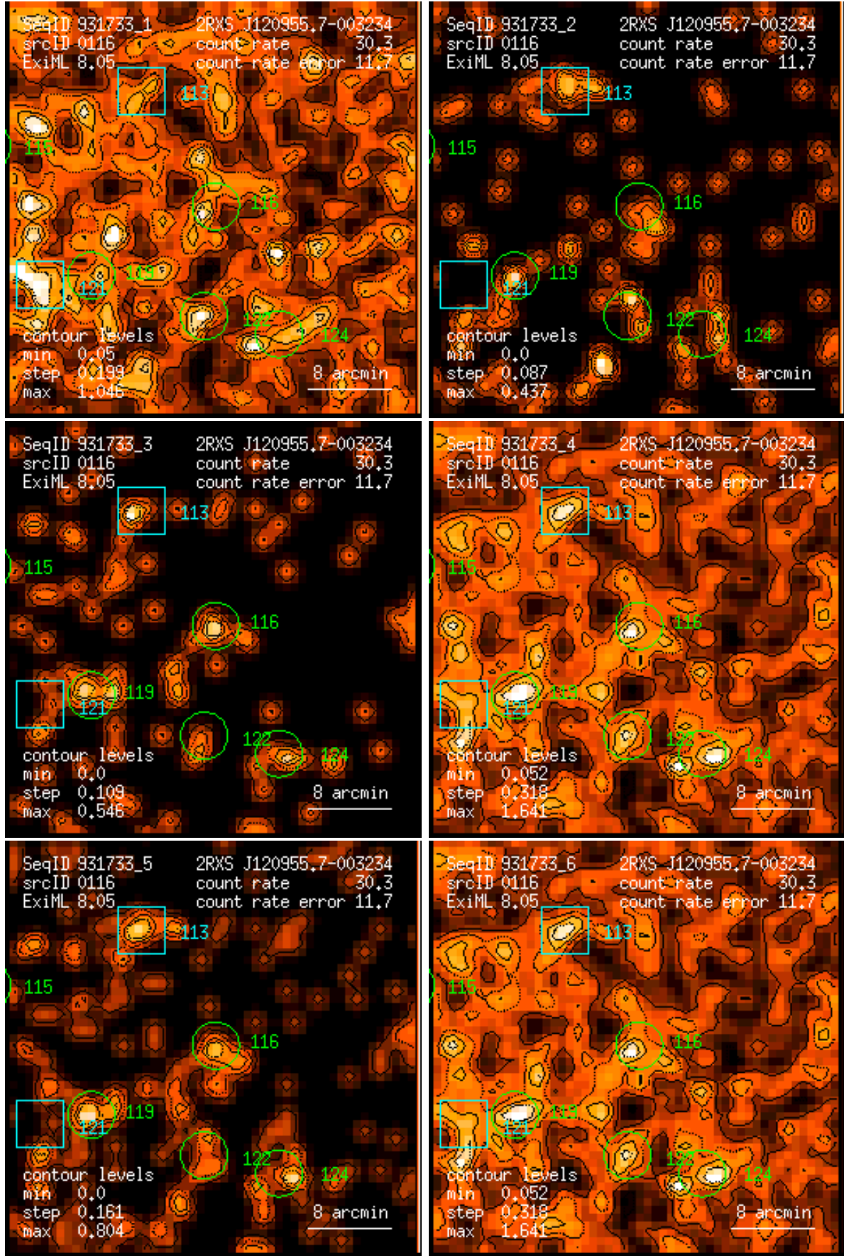
Figure 116: RASS 931733: detection 0116: band rate images, Gaussian filter: (1) PSPC channels 11 – 41, (2) 52 – 90, (3) 91 – 201, (4) 11 – 235, (5) 52 – 201, (6) 11 – 201. Broad band rates in counts/ks. Band rate contour levels in counts/ks/arcmin 2 .
