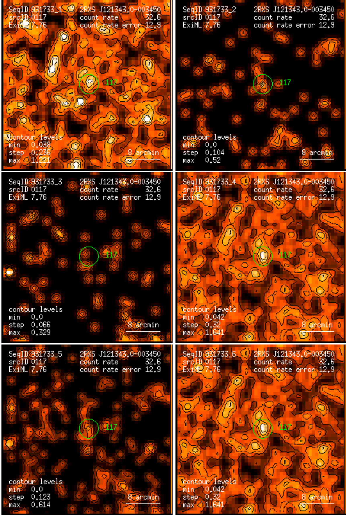
Figure 117: RASS 931733: detection 0117: band rate images, Gaussian filter: (1) PSPC channels 11 – 41, (2) 52 – 90, (3) 91 – 201, (4) 11 – 235, (5) 52 – 201, (6) 11 – 201. Broad band rates in counts/ks. Band rate contour levels in counts/ks/arcmin 2 .
