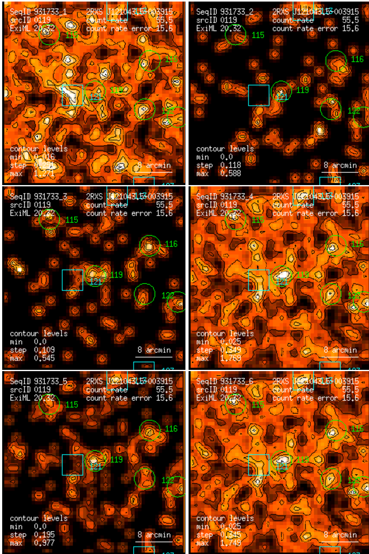
Figure 119: RASS 931733: detection 0119: band rate images, Gaussian filter: (1) PSPC channels 11 – 41, (2) 52 – 90, (3) 91 – 201, (4) 11 – 235, (5) 52 – 201, (6) 11 – 201. Broad band rates in counts/ks. Band rate contour levels in counts/ks/arcmin 2 .
