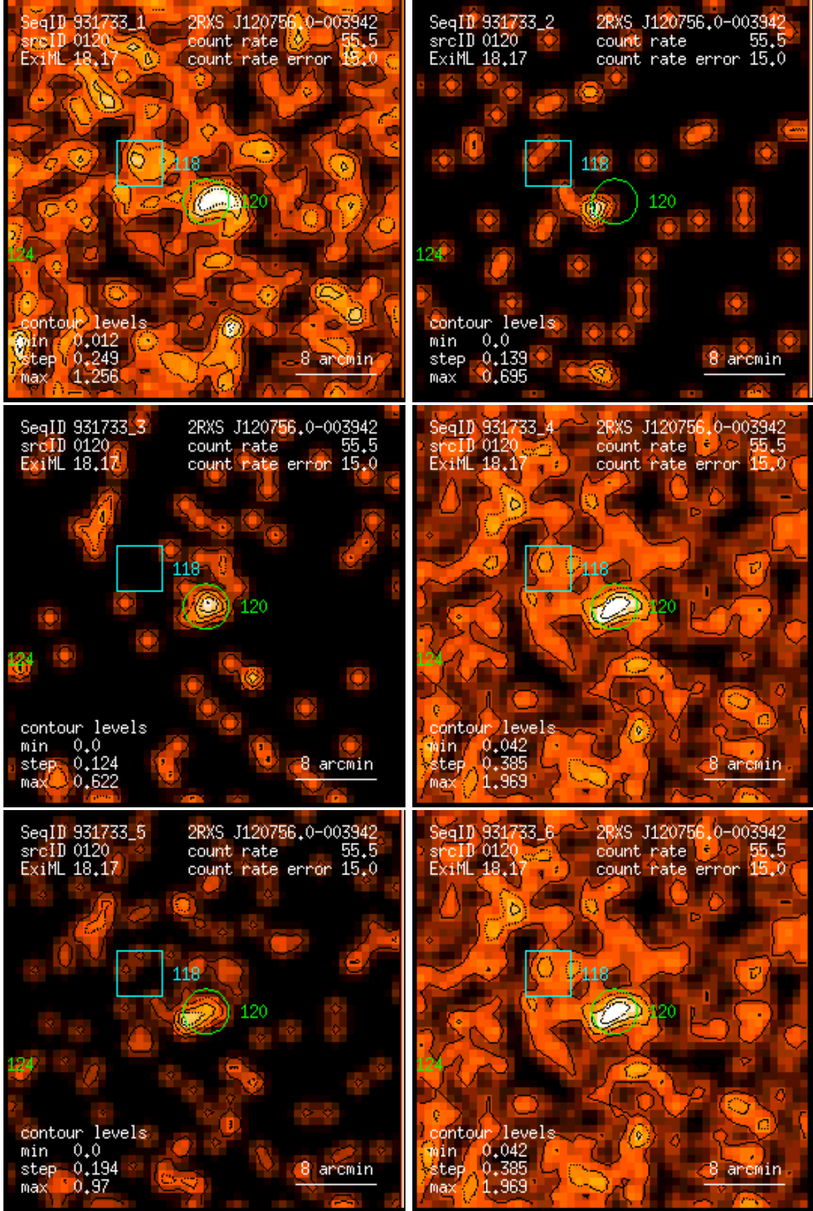
Figure 120: RASS 931733: detection 0120: band rate images, Gaussian filter: (1) PSPC channels 11 – 41, (2) 52 – 90, (3) 91 – 201, (4) 11 – 235, (5) 52 – 201, (6) 11 – 201. Broad band rates in counts/ks. Band rate contour levels in counts/ks/arcmin 2 .
