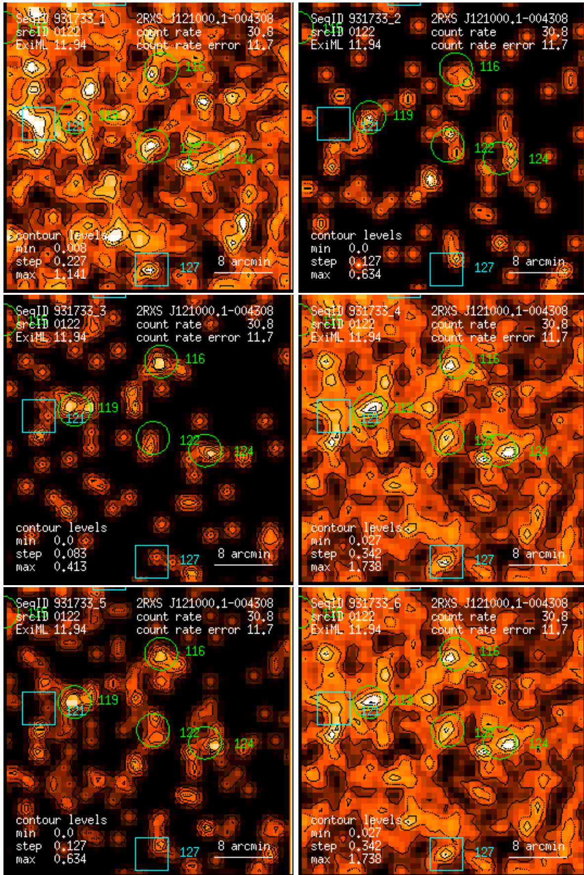
Figure 122: RASS 931733: detection 0122: band rate images, Gaussian filter: (1) PSPC channels 11 – 41, (2) 52 – 90, (3) 91 – 201, (4) 11 – 235, (5) 52 – 201, (6) 11 – 201. Broad band rates in counts/ks. Band rate contour levels in counts/ks/arcmin 2 .
