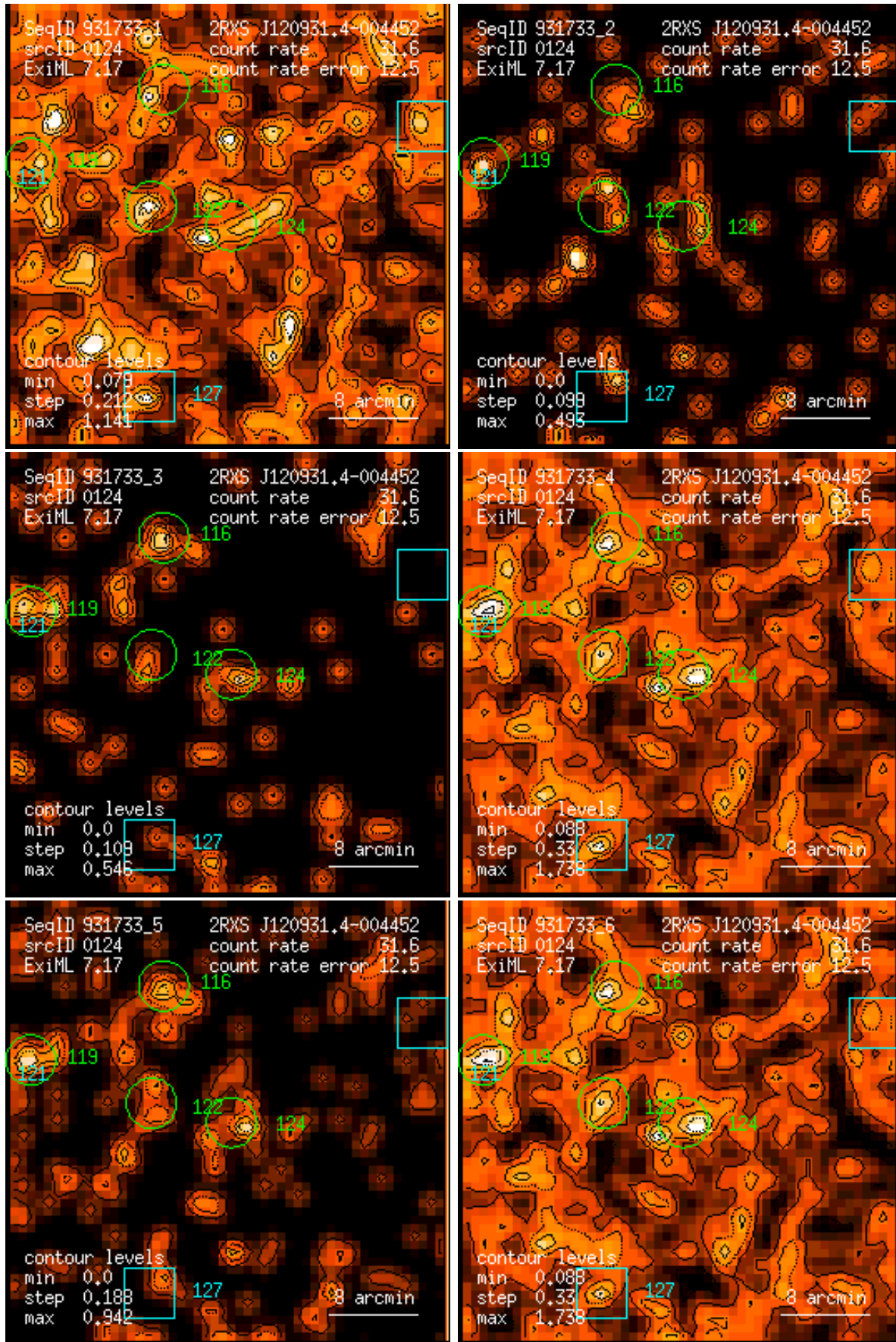
Figure 124: RASS 931733: detection 0124: band rate images, Gaussian filter: (1) PSPC channels 11 – 41, (2) 52 – 90, (3) 91 – 201, (4) 11 – 235, (5) 52 – 201, (6) 11 – 201. Broad band rates in counts/ks. Band rate contour levels in counts/ks/arcmin 2 .
