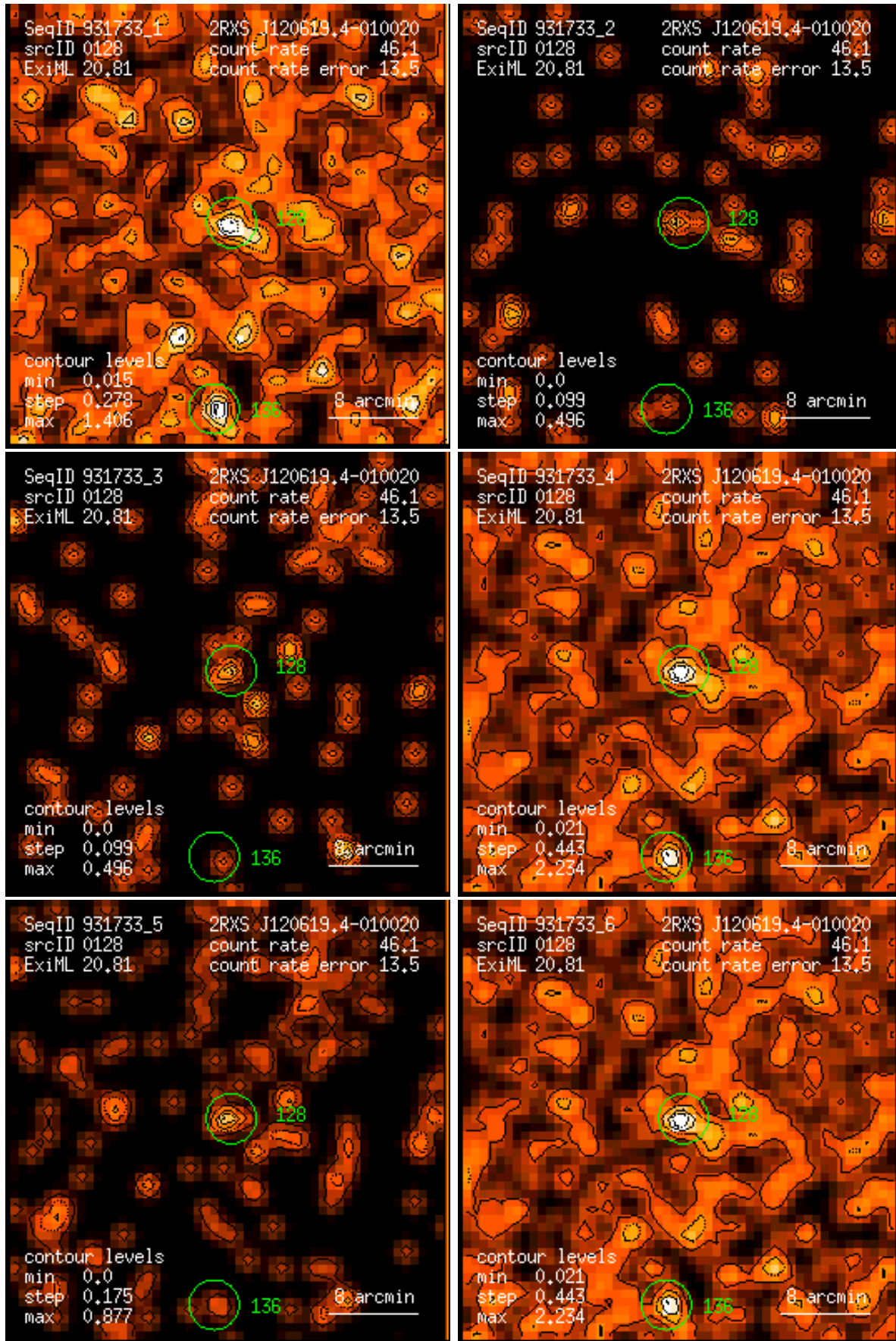
Figure 128: RASS 931733: detection 0128: band rate images, Gaussian filter: (1) PSPC channels 11 – 41, (2) 52 – 90, (3) 91 – 201, (4) 11 – 235, (5) 52 – 201, (6) 11 – 201. Broad band rates in counts/ks. Band rate contour levels in counts/ks/arcmin 2 .
