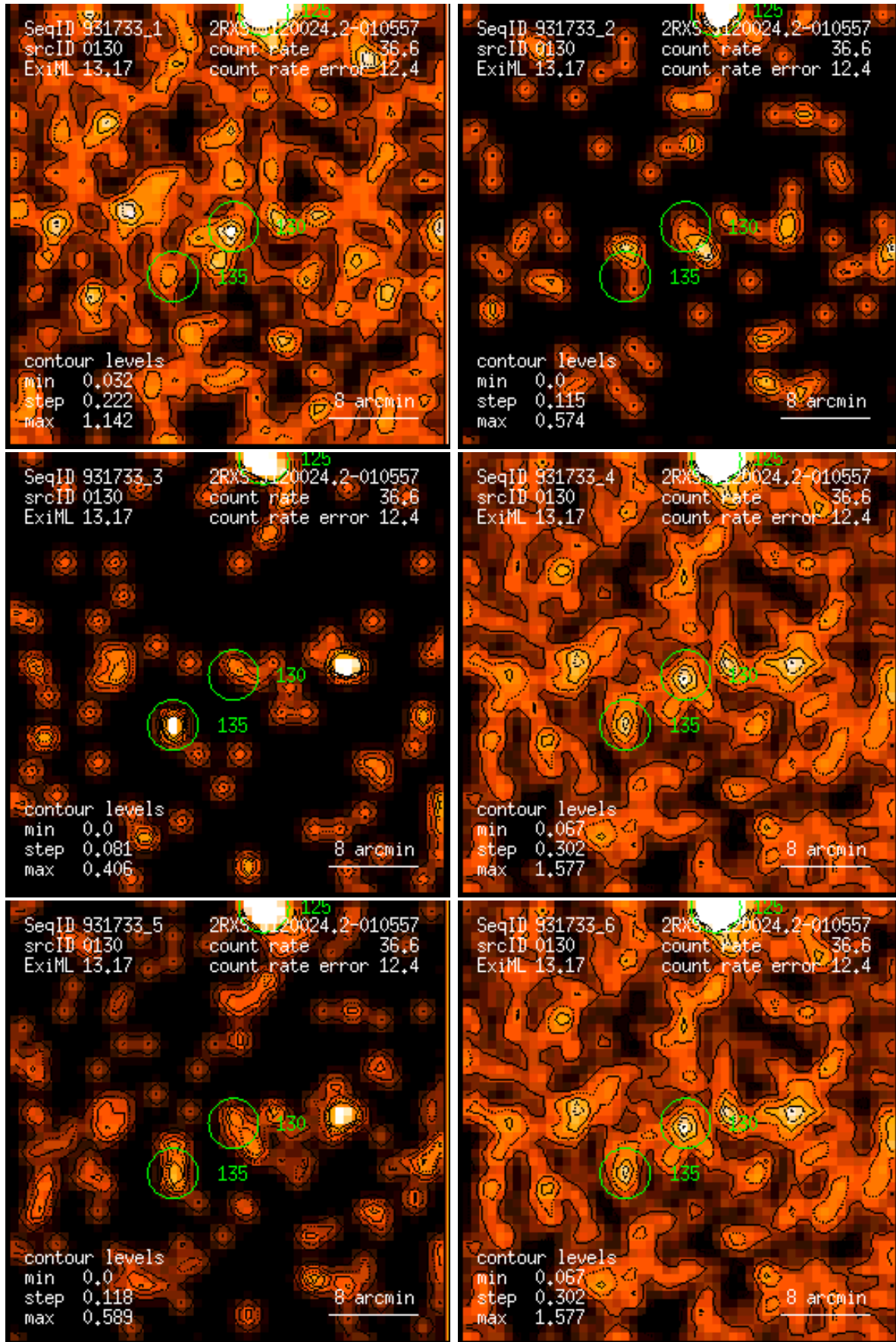
Figure 130: RASS 931733: detection 0130: band rate images, Gaussian filter: (1) PSPC channels 11 – 41, (2) 52 – 90, (3) 91 – 201, (4) 11 – 235, (5) 52 – 201, (6) 11 – 201. Broad band rates in counts/ks. Band rate contour levels in counts/ks/arcmin 2 .
