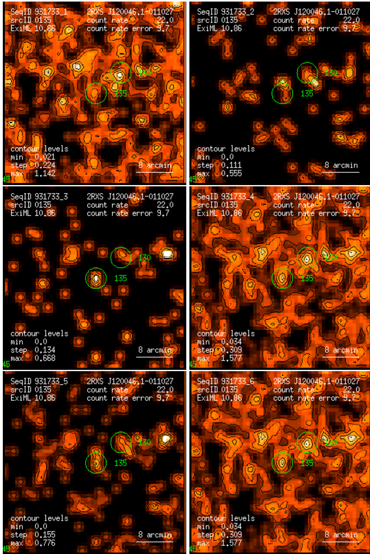
Figure 135: RASS 931733: detection 0135: band rate images, Gaussian filter: (1) PSPC channels 11 – 41, (2) 52 – 90, (3) 91 – 201, (4) 11 – 235, (5) 52 – 201, (6) 11 – 201. Broad band rates in counts/ks. Band rate contour levels in counts/ks/arcmin 2 .
