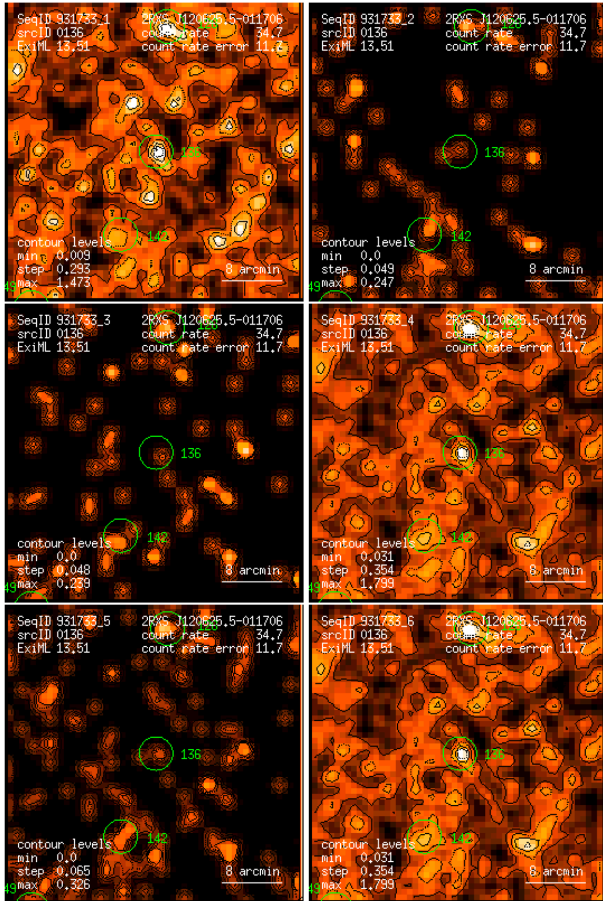
Figure 136: RASS 931733: detection 0136: band rate images, Gaussian filter: (1) PSPC channels 11 – 41, (2) 52 – 90, (3) 91 – 201, (4) 11 – 235, (5) 52 – 201, (6) 11 – 201. Broad band rates in counts/ks. Band rate contour levels in counts/ks/arcmin 2 .
