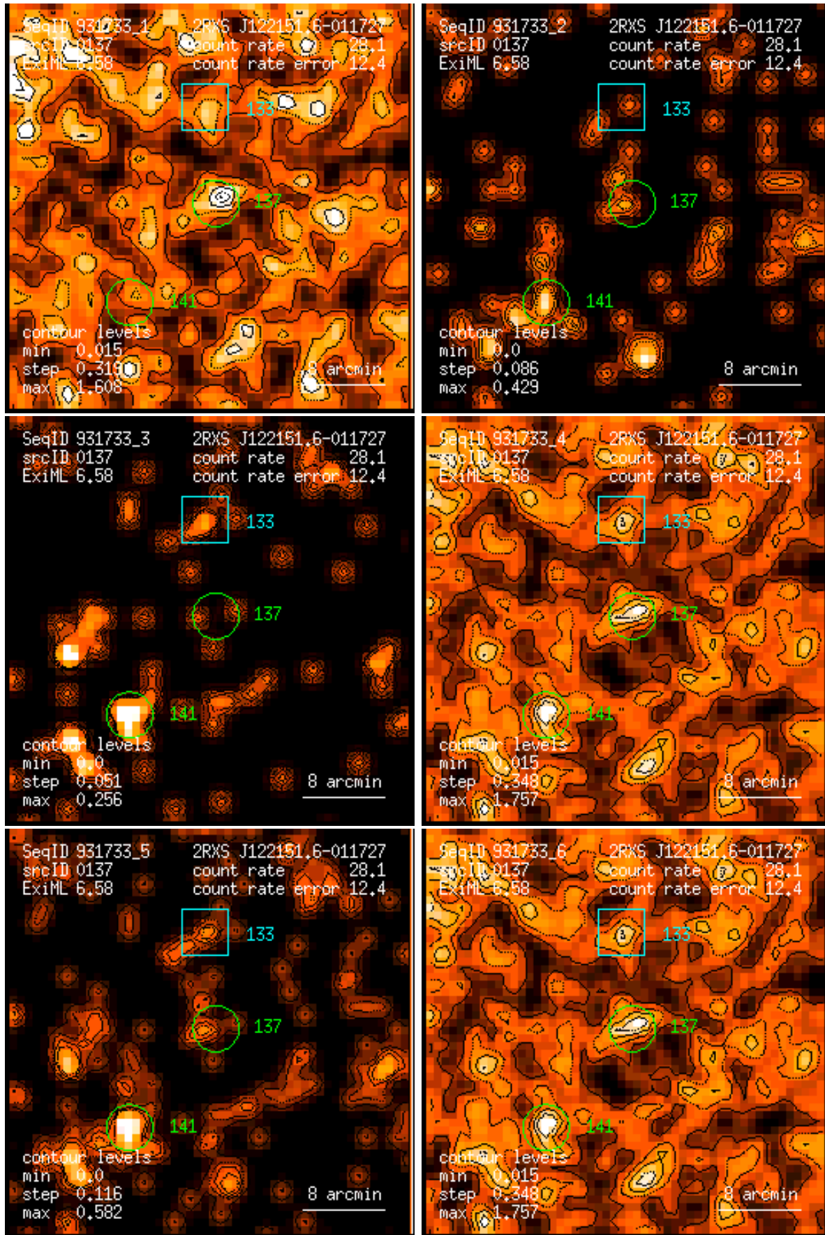
Figure 137: RASS 931733: detection 0137: band rate images, Gaussian filter: (1) PSPC channels 11 – 41, (2) 52 – 90, (3) 91 – 201, (4) 11 – 235, (5) 52 – 201, (6) 11 – 201. Broad band rates in counts/ks. Band rate contour levels in counts/ks/arcmin 2 .
