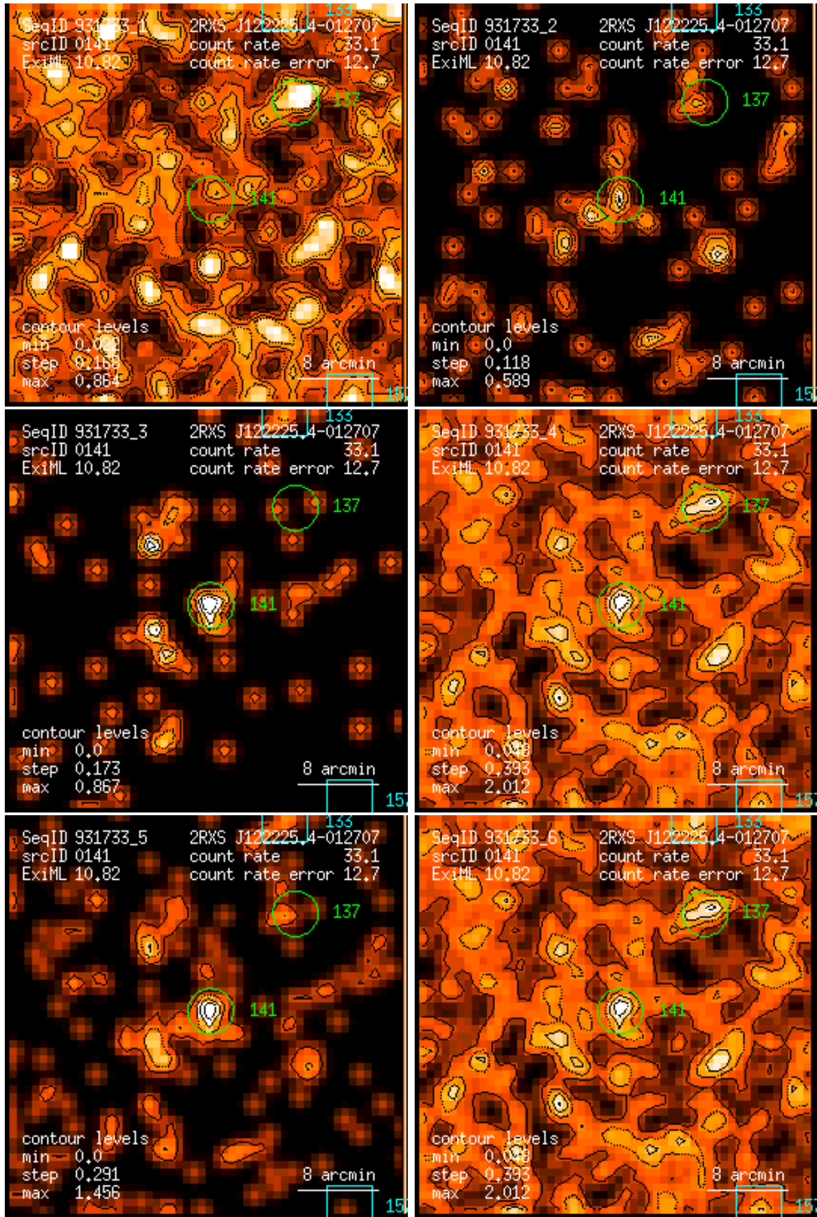
Figure 141: RASS 931733: detection 0141: band rate images, Gaussian filter: (1) PSPC channels 11 – 41, (2) 52 – 90, (3) 91 – 201, (4) 11 – 235, (5) 52 – 201, (6) 11 – 201. Broad band rates in counts/ks. Band rate contour levels in counts/ks/arcmin 2 .
