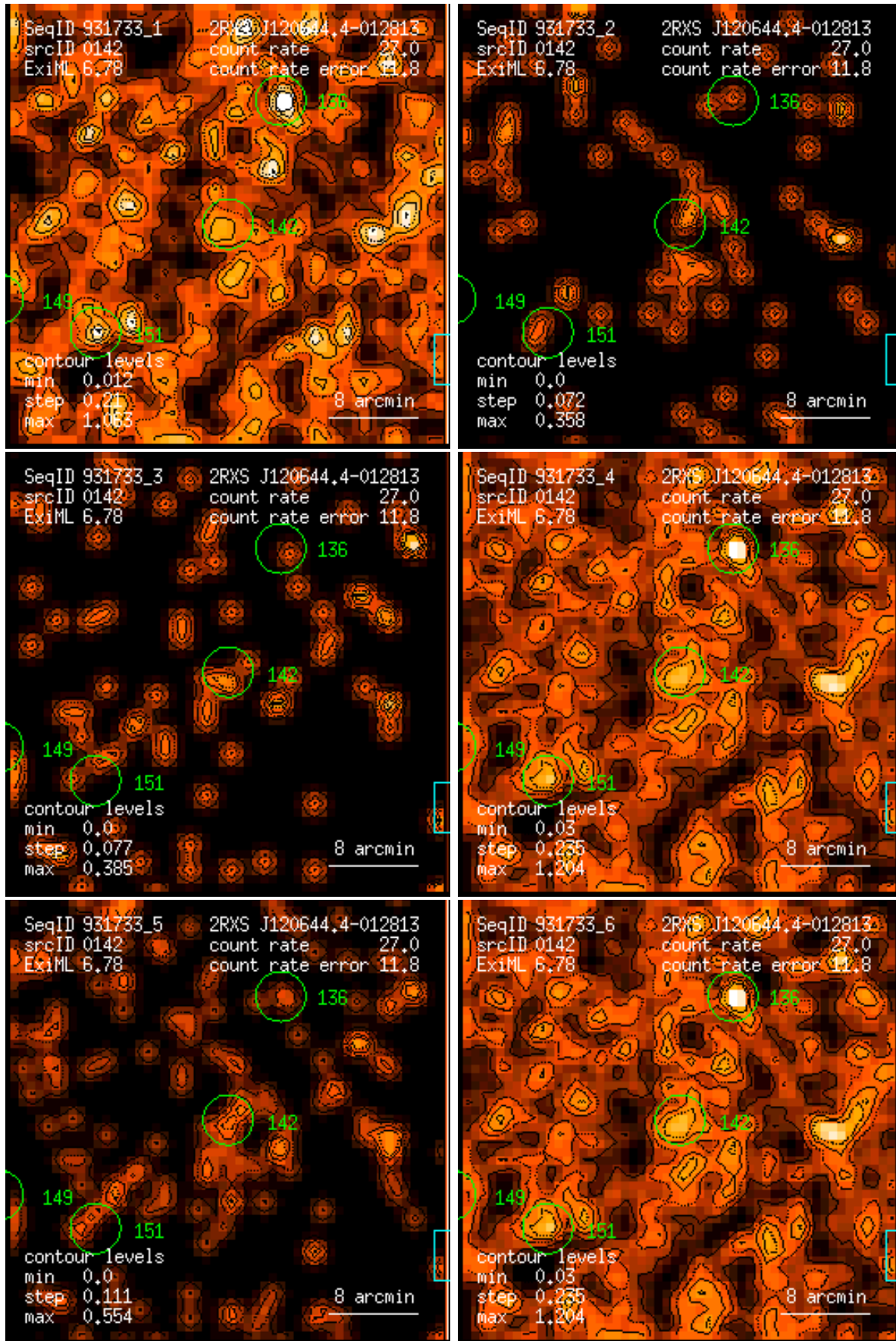
Figure 142: RASS 931733: detection 0142: band rate images, Gaussian filter: (1) PSPC channels 11 – 41, (2) 52 – 90, (3) 91 – 201, (4) 11 – 235, (5) 52 – 201, (6) 11 – 201. Broad band rates in counts/ks. Band rate contour levels in counts/ks/arcmin 2 .
