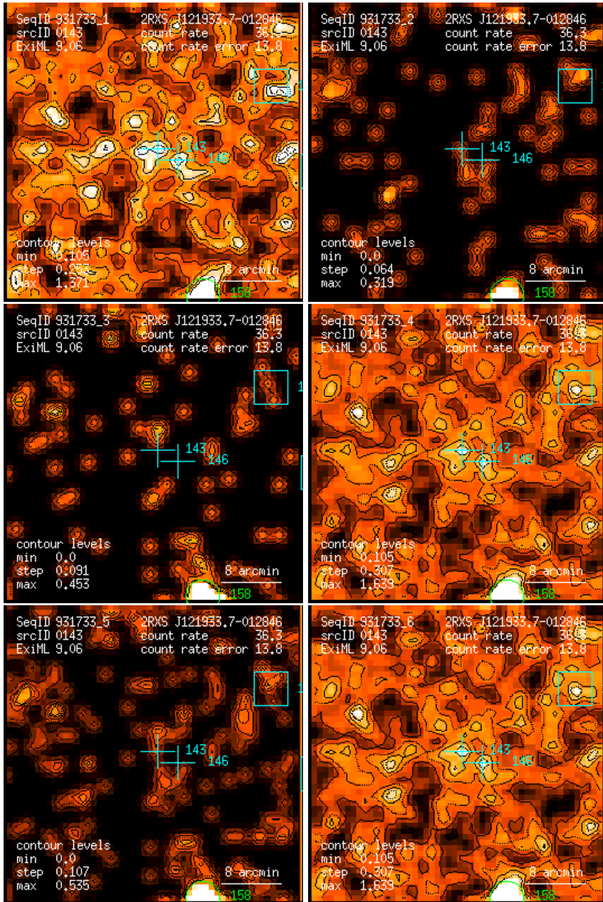
Figure 143: RASS 931733: detection 0143: band rate images, Gaussian filter: (1) PSPC channels 11 – 41, (2) 52 – 90, (3) 91 – 201, (4) 11 – 235, (5) 52 – 201, (6) 11 – 201. Broad band rates in counts/ks. Band rate contour levels in counts/ks/arcmin 2 .
