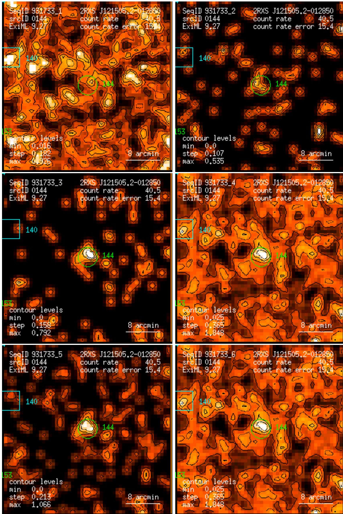
Figure 144: RASS 931733: detection 0144: band rate images, Gaussian filter: (1) PSPC channels 11 – 41, (2) 52 – 90, (3) 91 – 201, (4) 11 – 235, (5) 52 – 201, (6) 11 – 201. Broad band rates in counts/ks. Band rate contour levels in counts/ks/arcmin 2 .
