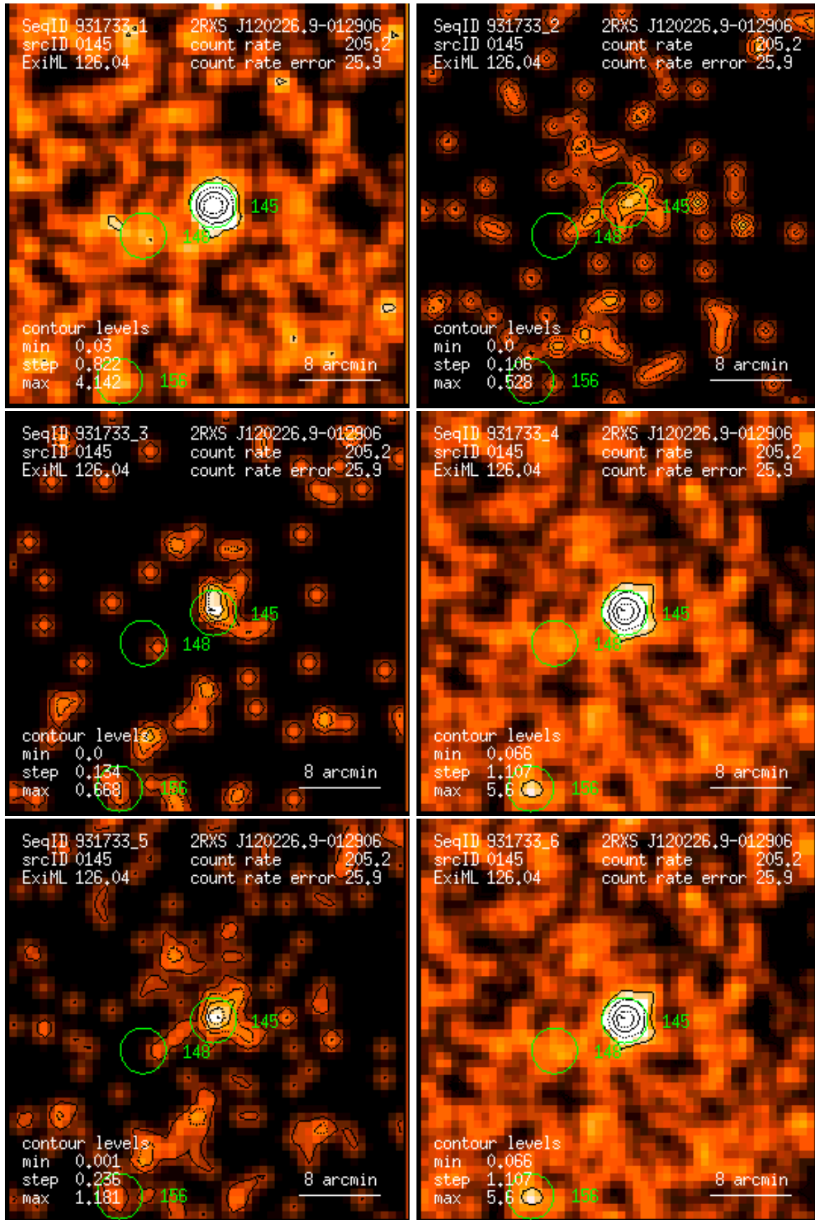
Figure 145: RASS 931733: detection 0145: band rate images, Gaussian filter: (1) PSPC channels 11 – 41, (2) 52 – 90, (3) 91 – 201, (4) 11 – 235, (5) 52 – 201, (6) 11 – 201. Broad band rates in counts/ks. Band rate contour levels in counts/ks/arcmin 2 .
