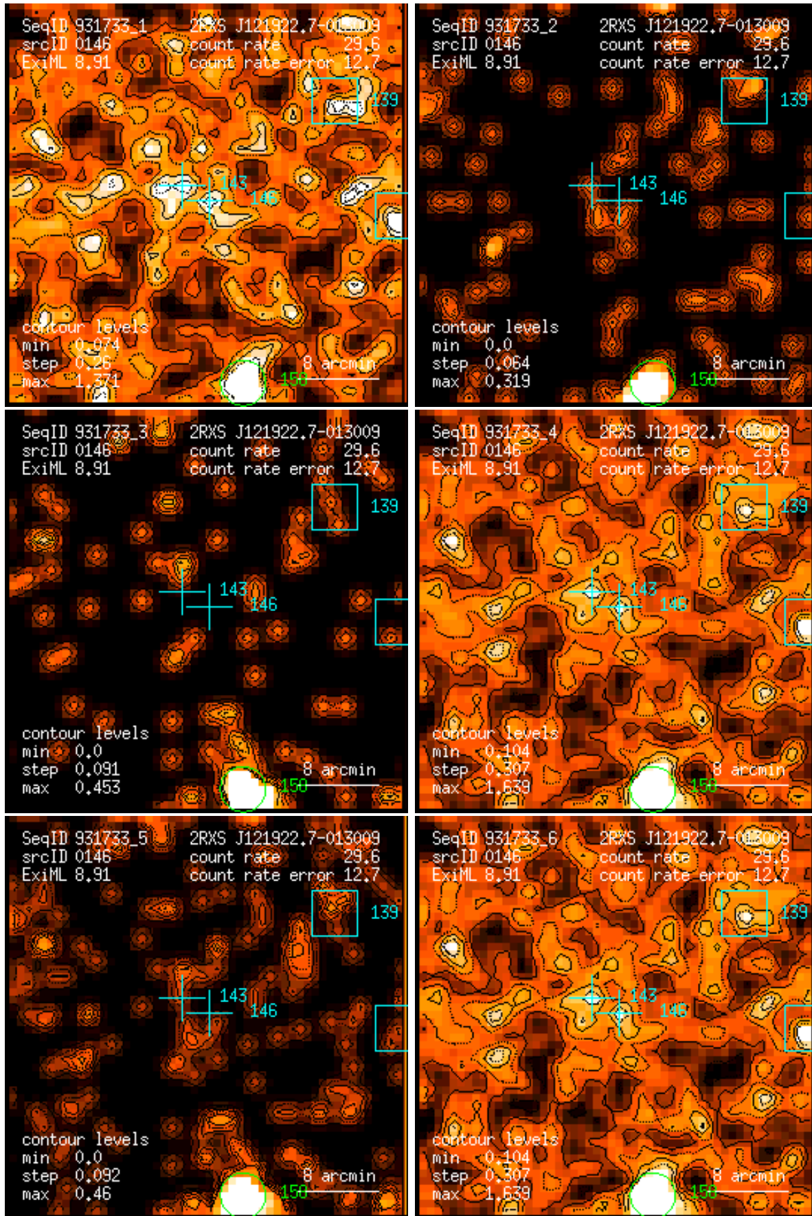
Figure 146: RASS 931733: detection 0146: band rate images, Gaussian filter: (1) PSPC channels 11 – 41, (2) 52 – 90, (3) 91 – 201, (4) 11 – 235, (5) 52 – 201, (6) 11 – 201. Broad band rates in counts/ks. Band rate contour levels in counts/ks/arcmin 2 .
