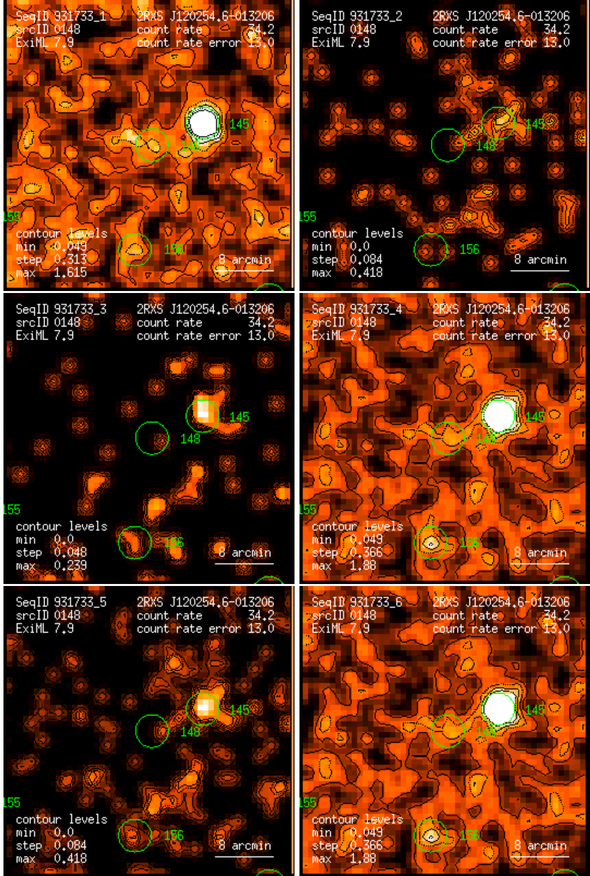
Figure 148: RASS 931733: detection 0148: band rate images, Gaussian filter: (1) PSPC channels 11 – 41, (2) 52 – 90, (3) 91 – 201, (4) 11 – 235, (5) 52 – 201, (6) 11 – 201. Broad band rates in counts/ks. Band rate contour levels in counts/ks/arcmin 2 .
