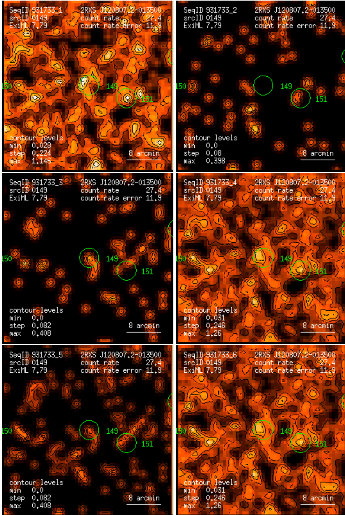
Figure 149: RASS 931733: detection 0149: band rate images, Gaussian filter: (1) PSPC channels 11 – 41, (2) 52 – 90, (3) 91 – 201, (4) 11 – 235, (5) 52 – 201, (6) 11 – 201. Broad band rates in counts/ks. Band rate contour levels in counts/ks/arcmin 2 .
