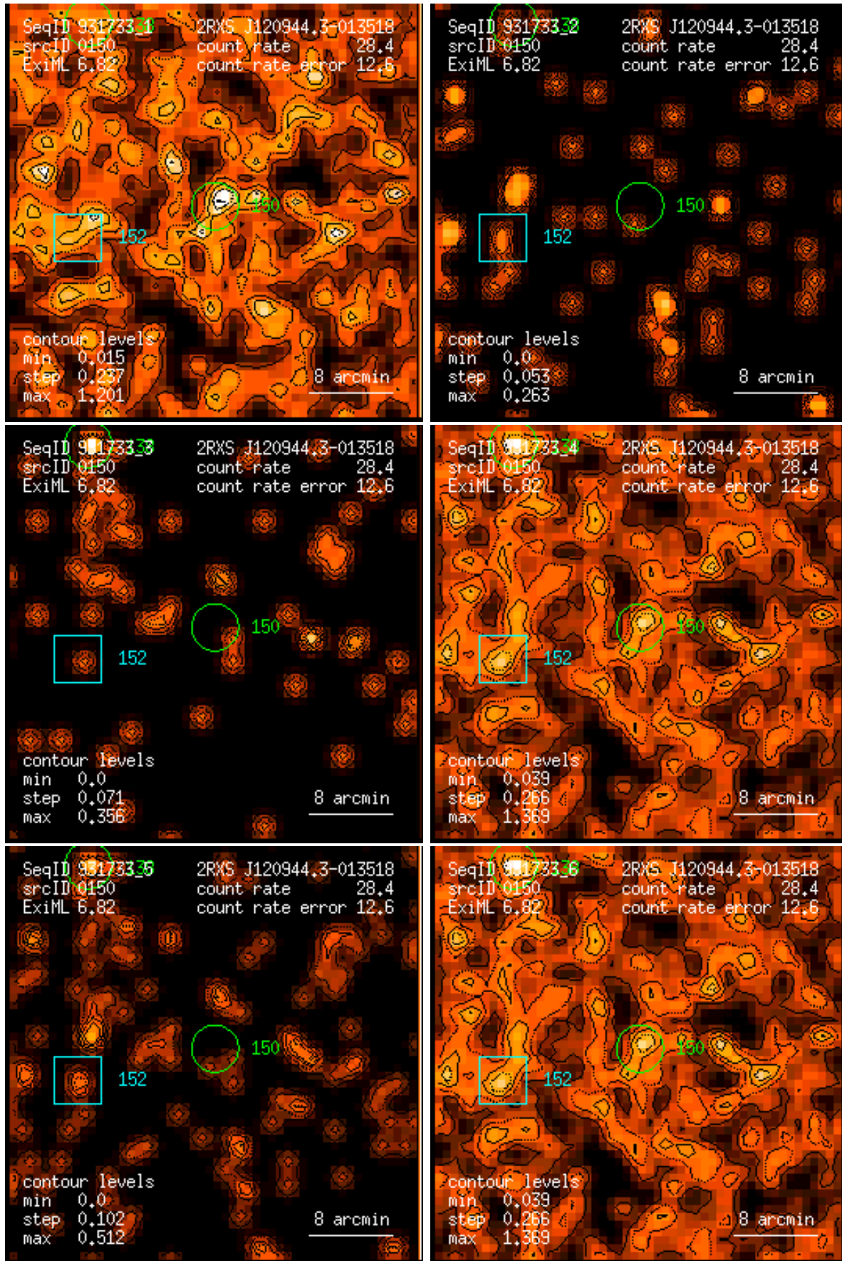
Figure 150: RASS 931733: detection 0150: band rate images, Gaussian filter: (1) PSPC channels 11 – 41, (2) 52 – 90, (3) 91 – 201, (4) 11 – 235, (5) 52 – 201, (6) 11 – 201. Broad band rates in counts/ks. Band rate contour levels in counts/ks/arcmin 2 .
