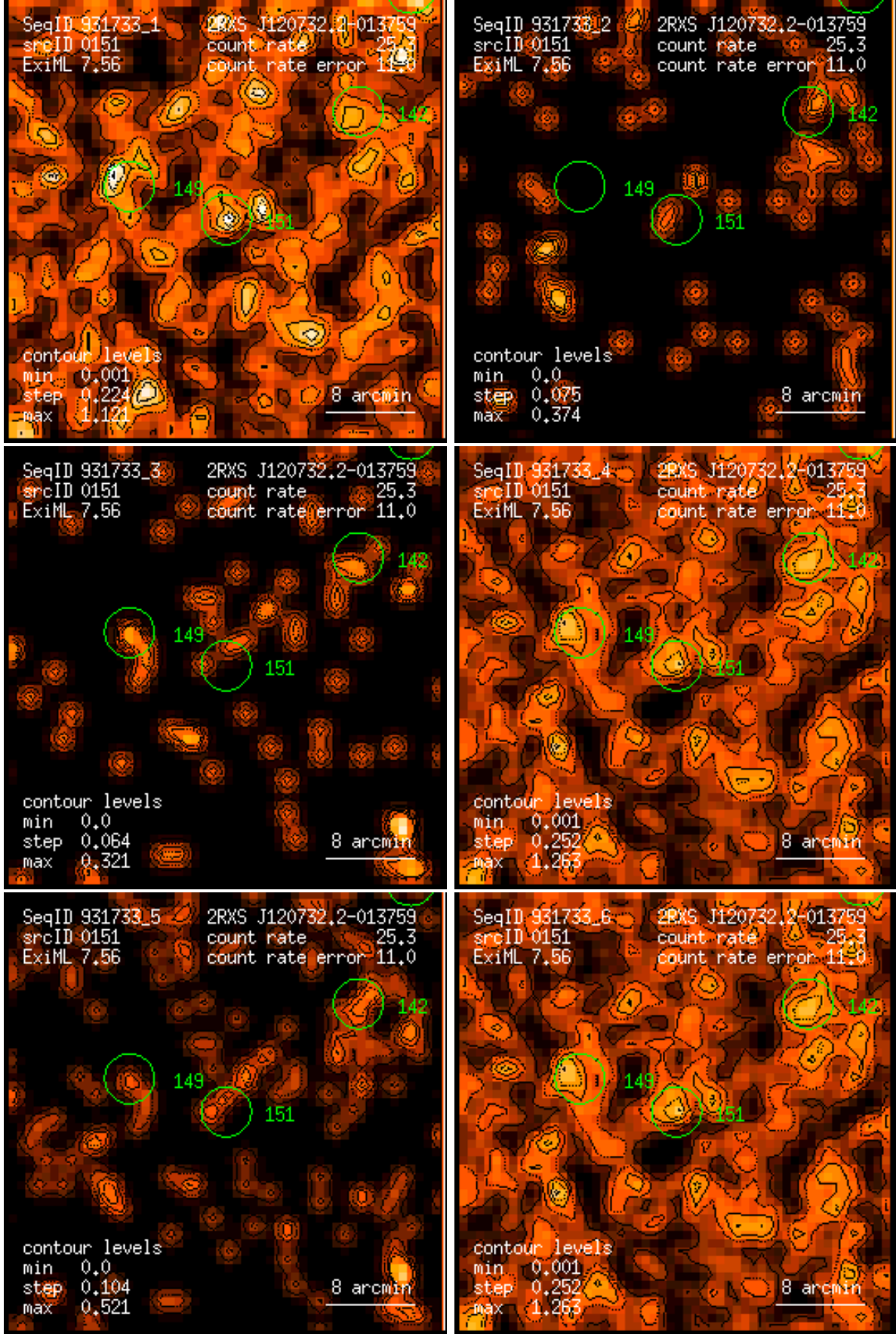
Figure 151: RASS 931733: detection 0151: band rate images, Gaussian filter: (1) PSPC channels 11 – 41, (2) 52 – 90, (3) 91 – 201, (4) 11 – 235, (5) 52 – 201, (6) 11 – 201. Broad band rates in counts/ks. Band rate contour levels in counts/ks/arcmin 2 .
