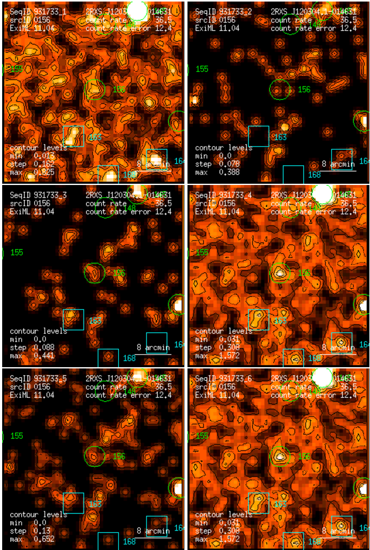
Figure 156: RASS 931733: detection 0156: band rate images, Gaussian filter: (1) PSPC channels 11 – 41, (2) 52 – 90, (3) 91 – 201, (4) 11 – 235, (5) 52 – 201, (6) 11 – 201. Broad band rates in counts/ks. Band rate contour levels in counts/ks/arcmin 2 .
