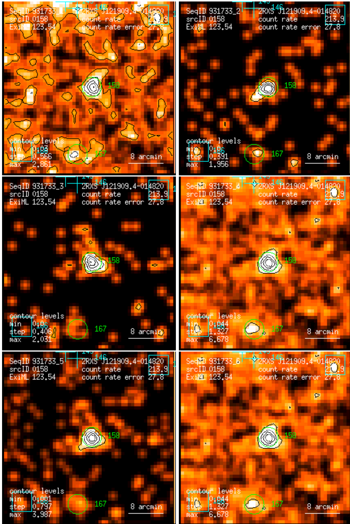
Figure 158: RASS 931733: detection 0158: band rate images, Gaussian filter: (1) PSPC channels 11 – 41, (2) 52 – 90, (3) 91 – 201, (4) 11 – 235, (5) 52 – 201, (6) 11 – 201. Broad band rates in counts/ks. Band rate contour levels in counts/ks/arcmin 2 .
