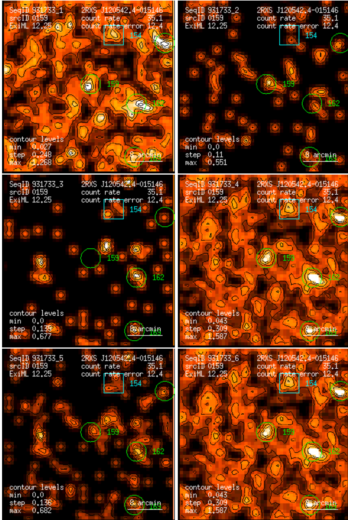
Figure 159: RASS 931733: detection 0159: band rate images, Gaussian filter: (1) PSPC channels 11 – 41, (2) 52 – 90, (3) 91 – 201, (4) 11 – 235, (5) 52 – 201, (6) 11 – 201. Broad band rates in counts/ks. Band rate contour levels in counts/ks/arcmin 2 .
