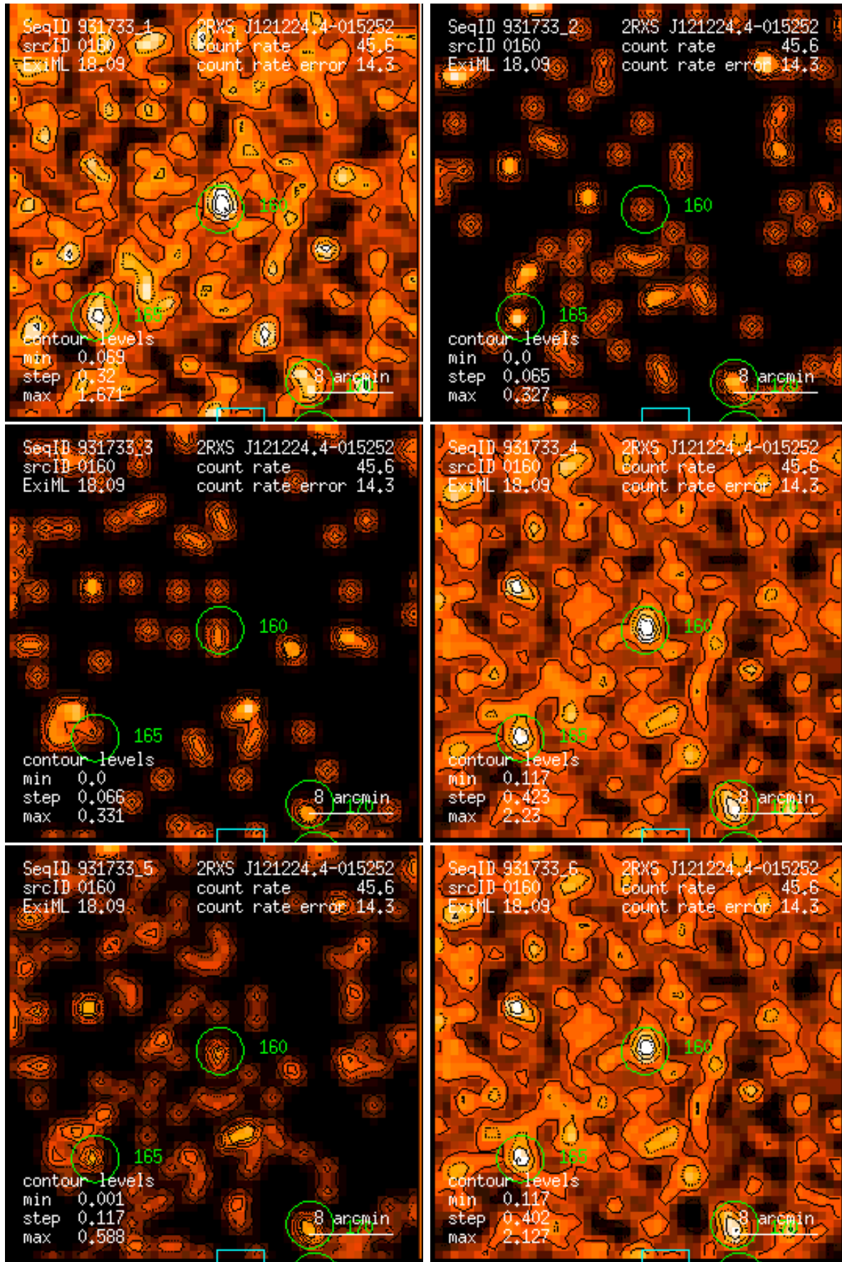
Figure 160: RASS 931733: detection 0160: band rate images, Gaussian filter: (1) PSPC channels 11 – 41, (2) 52 – 90, (3) 91 – 201, (4) 11 – 235, (5) 52 – 201, (6) 11 – 201. Broad band rates in counts/ks. Band rate contour levels in counts/ks/arcmin 2 .
