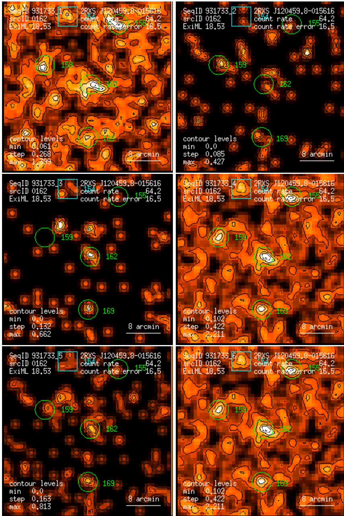
Figure 162: RASS 931733: detection 0162: band rate images, Gaussian filter: (1) PSPC channels 11 – 41, (2) 52 – 90, (3) 91 – 201, (4) 11 – 235, (5) 52 – 201, (6) 11 – 201. Broad band rates in counts/ks. Band rate contour levels in counts/ks/arcmin 2 .
