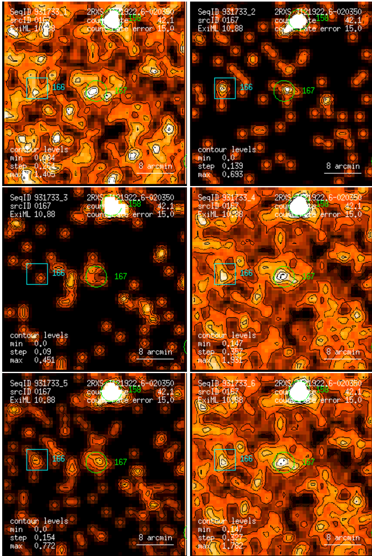
Figure 167: RASS 931733: detection 0167: band rate images, Gaussian filter: (1) PSPC channels 11 – 41, (2) 52 – 90, (3) 91 – 201, (4) 11 – 235, (5) 52 – 201, (6) 11 – 201. Broad band rates in counts/ks. Band rate contour levels in counts/ks/arcmin 2 .
