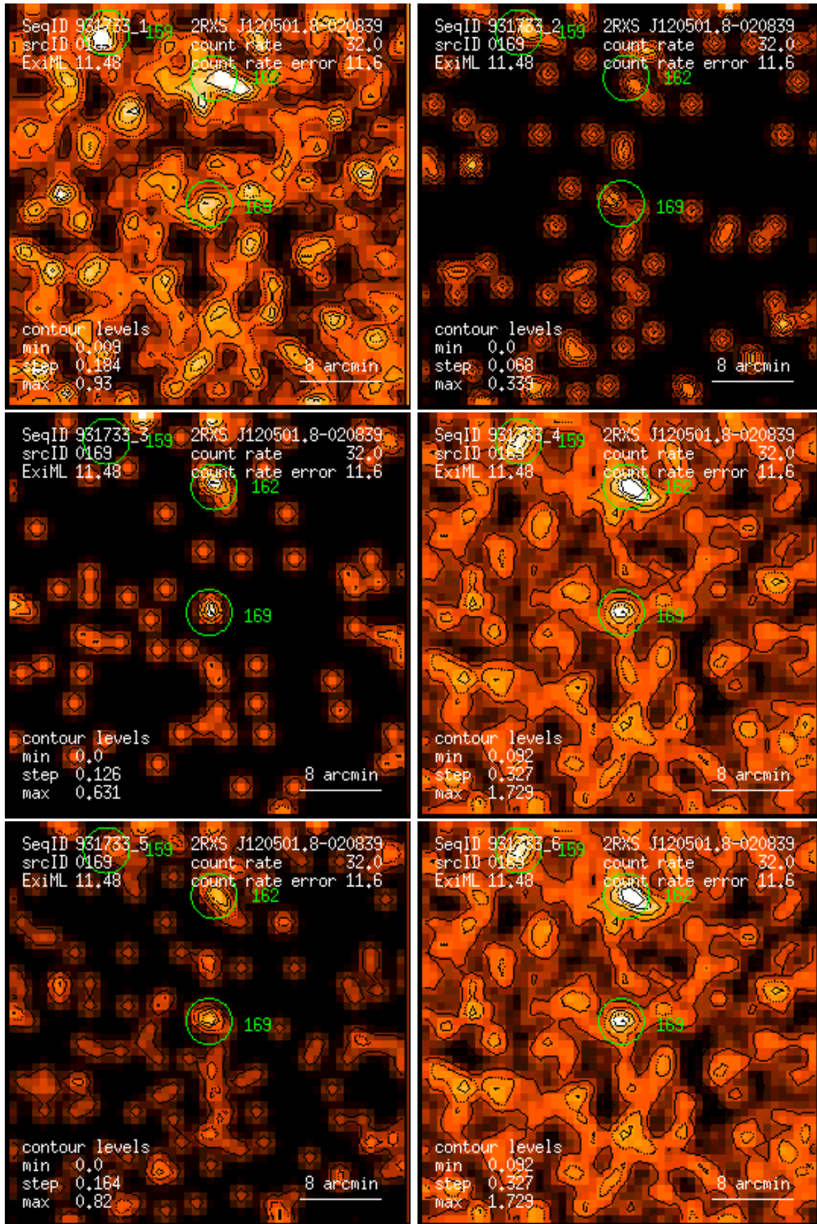
Figure 169: RASS 931733: detection 0169: band rate images, Gaussian filter: (1) PSPC channels 11 – 41, (2) 52 – 90, (3) 91 – 201, (4) 11 – 235, (5) 52 – 201, (6) 11 – 201. Broad band rates in counts/ks. Band rate contour levels in counts/ks/arcmin 2 .
