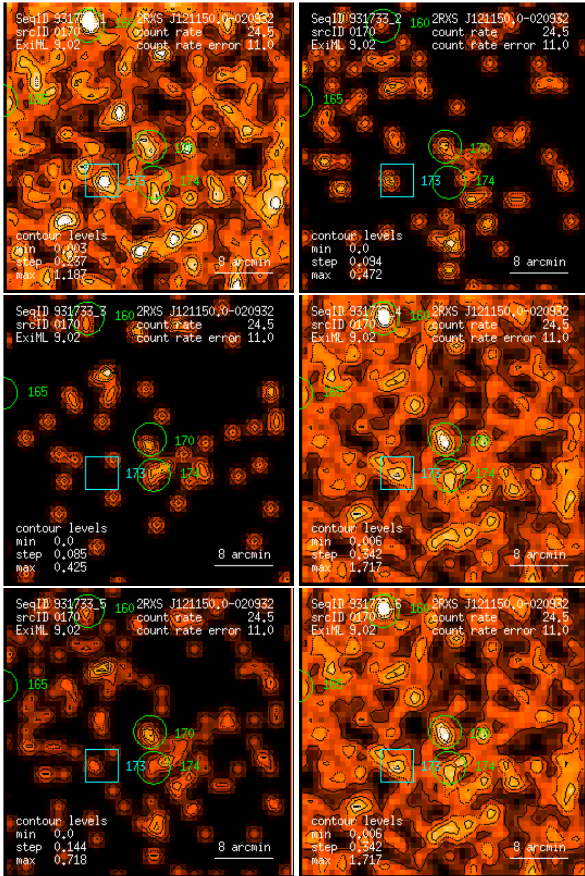
Figure 170: RASS 931733: detection 0170: band rate images, Gaussian filter: (1) PSPC channels 11 – 41, (2) 52 – 90, (3) 91 – 201, (4) 11 – 235, (5) 52 – 201, (6) 11 – 201. Broad band rates in counts/ks. Band rate contour levels in counts/ks/arcmin 2 .
