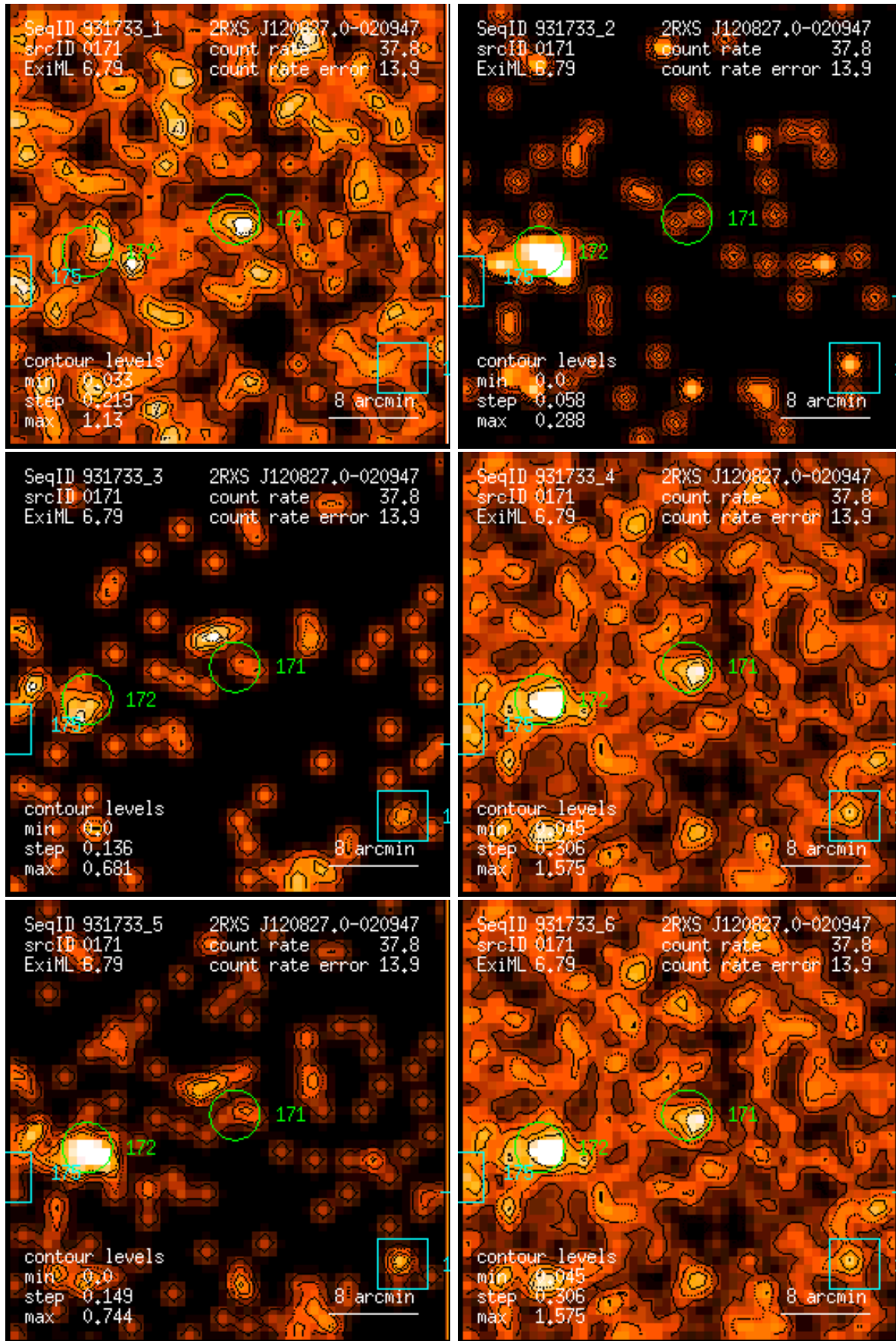
Figure 171: RASS 931733: detection 0171: band rate images, Gaussian filter: (1) PSPC channels 11 – 41, (2) 52 – 90, (3) 91 – 201, (4) 11 – 235, (5) 52 – 201, (6) 11 – 201. Broad band rates in counts/ks. Band rate contour levels in counts/ks/arcmin 2 .
